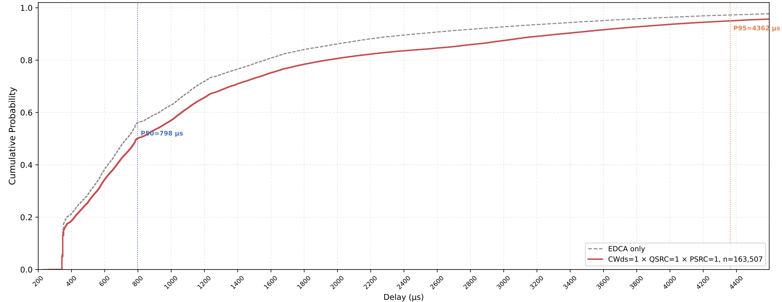
VO (all STAs) Delay CDF — CWds=1 × QSRC=1 × PSRC=1 nSta=30, nPedca=30, 0.5Mbps, avg of 10 runs
