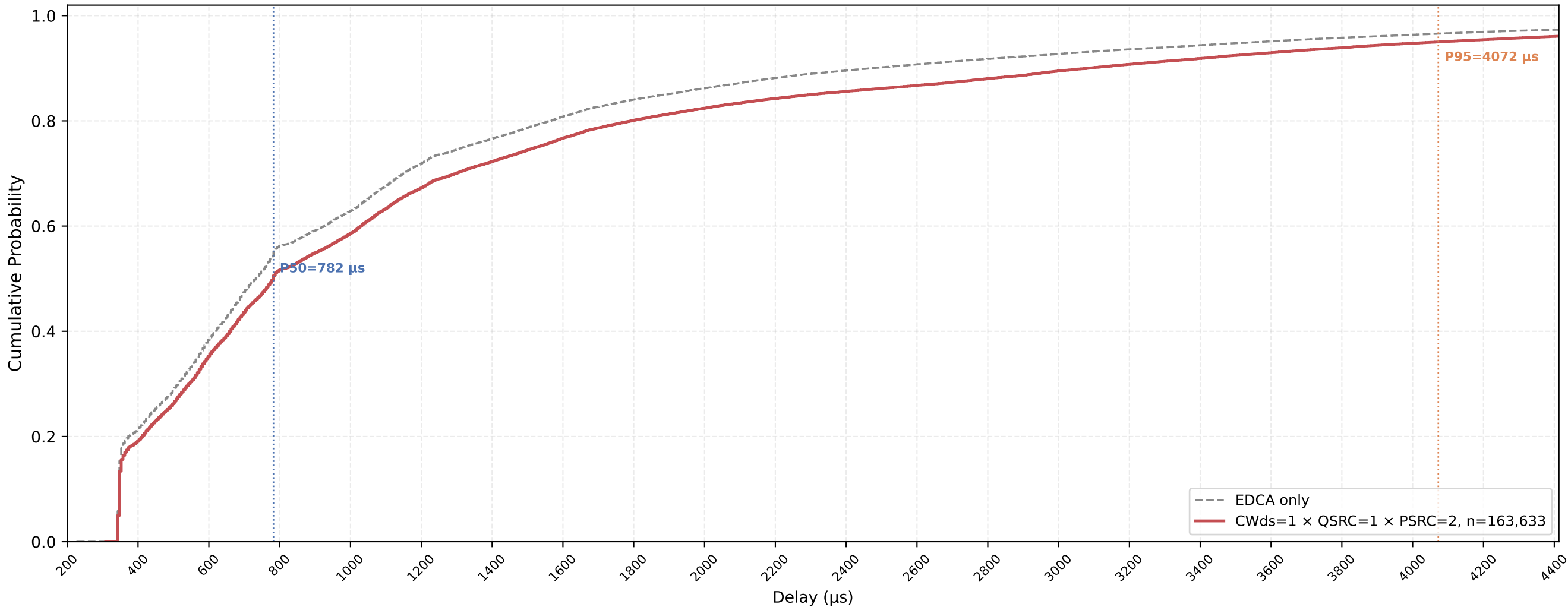
VO (all STAs) Delay CDF — CWds=1 × QSRC=1 × PSRC=2 nSta=30, nPedca=15, 0.5Mbps, avg of 10 runs
