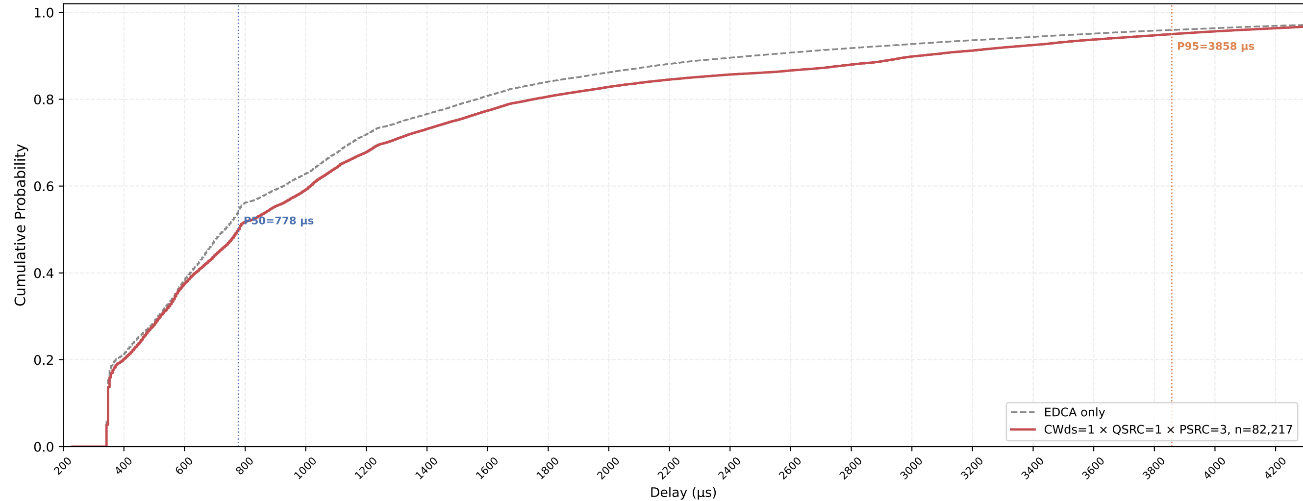
P-EDCA STA VO Delay CDF — CWds=1 × QSRC=1 × PSRC=3 nSta=30, nPedca=15, 0.5Mbps, avg of 10 runs
