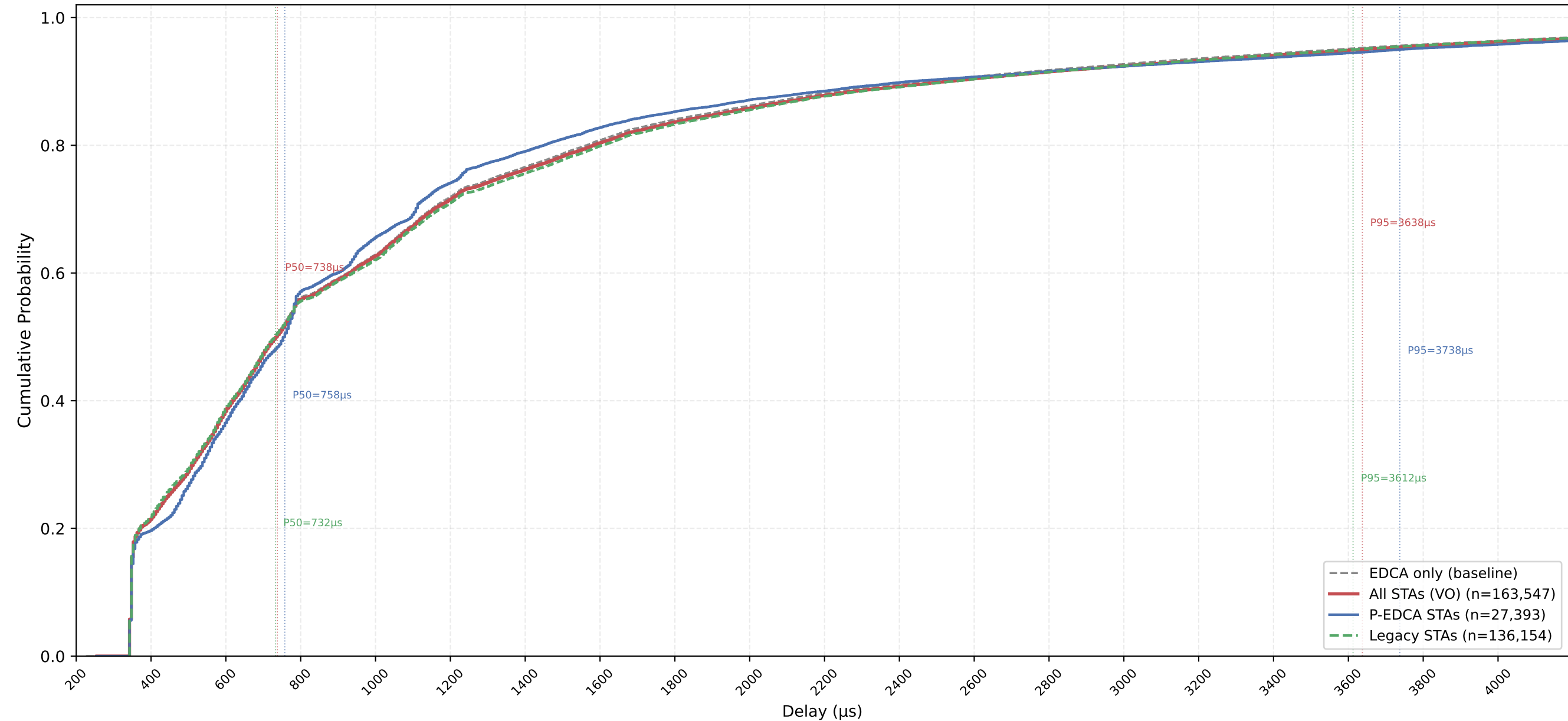
VO Delay CDF — P-EDCA / Legacy / All | CWds=1 × QSRC=2 × PSRC=1 nSta=30, nPedca=5/30, 0.5Mbps, avg of 10 runs
