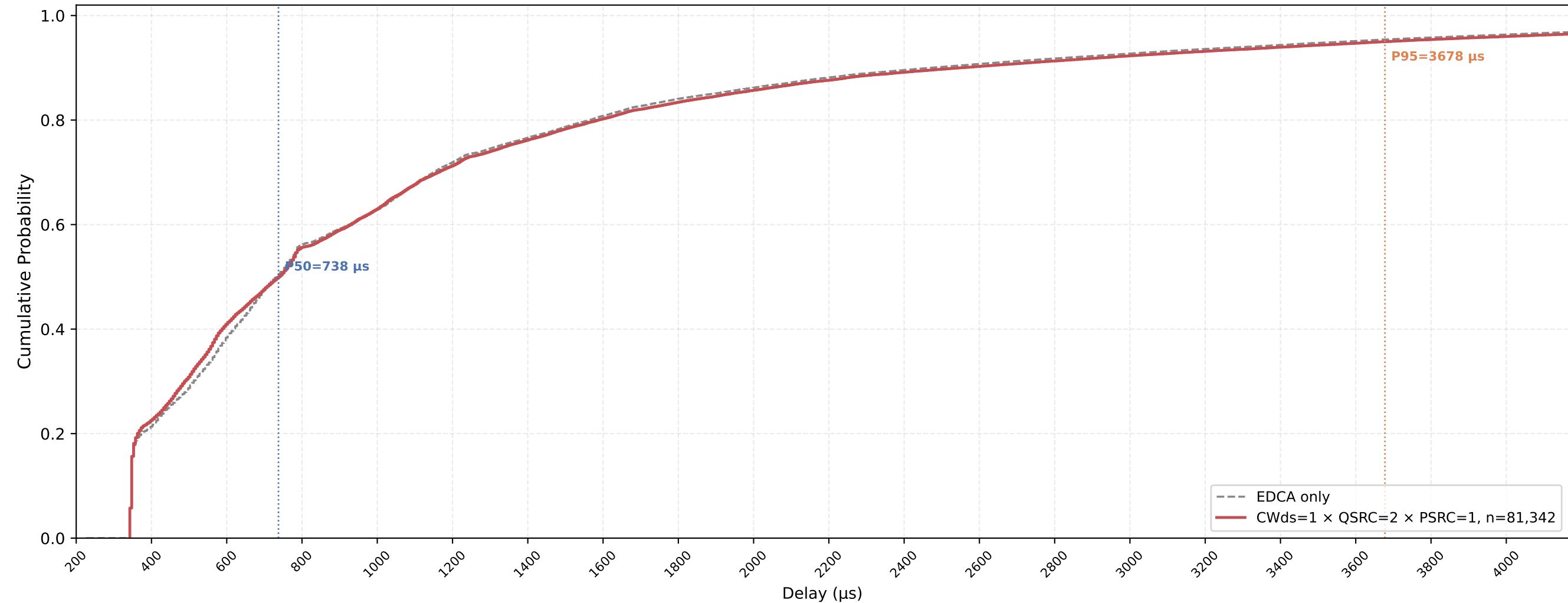
P-EDCA STA VO Delay CDF — CWds=1 × QSRC=2 × PSRC=1 nSta=30, nPedca=15, 0.5Mbps, avg of 10 runs
