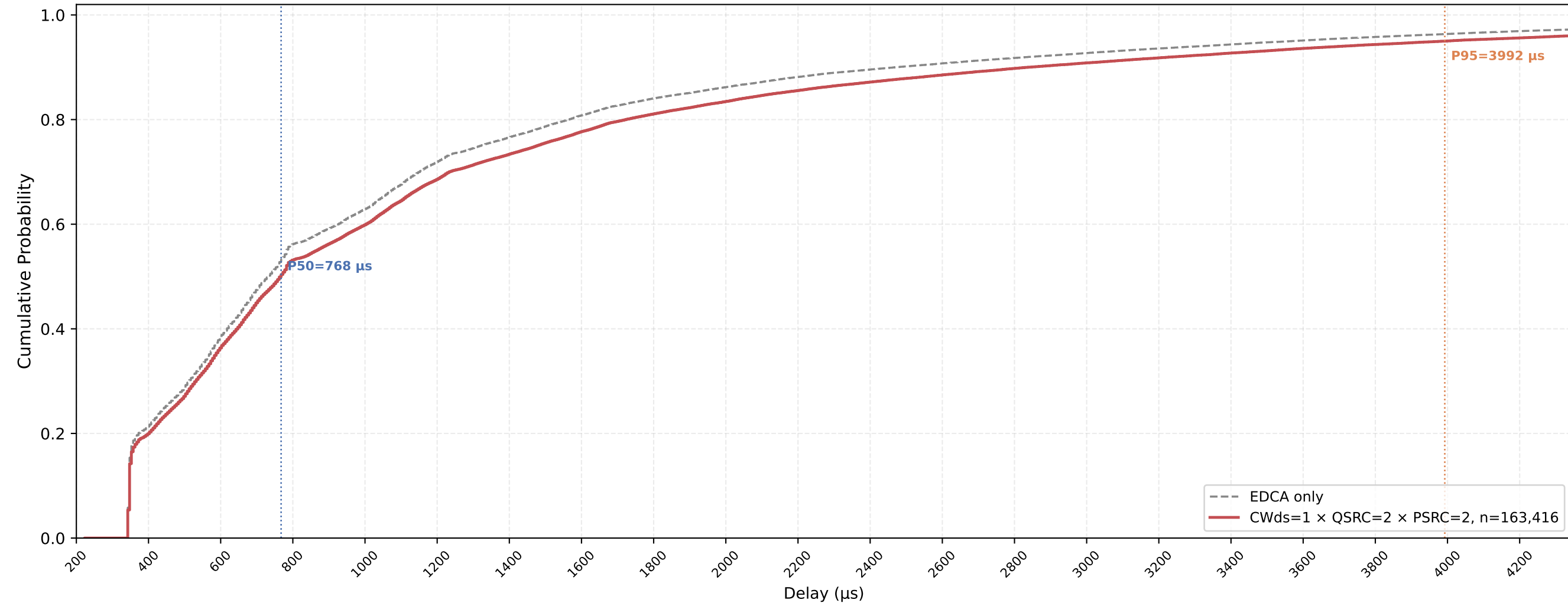
VO (all STAs) Delay CDF — CWds=1 × QSRC=2 × PSRC=2 nSta=30, nPedca=30, 0.5Mbps, avg of 10 runs
