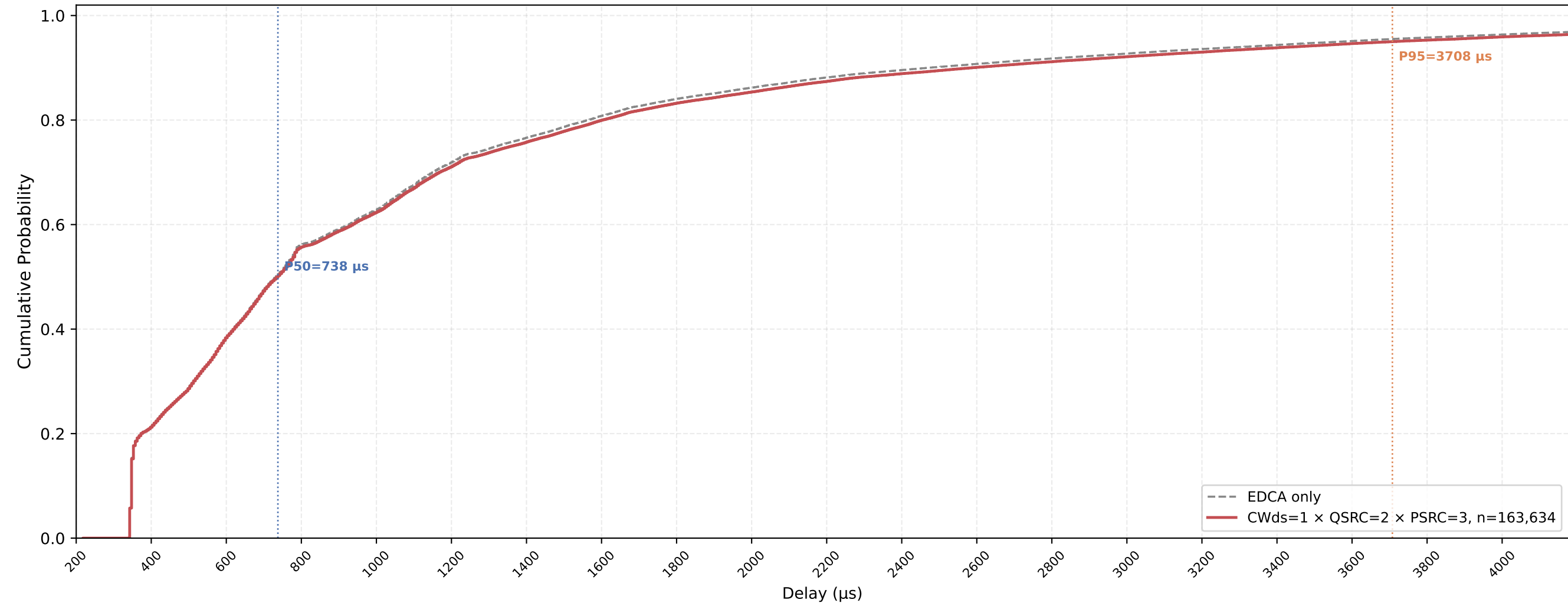
VO (all STAs) Delay CDF — CWds=1 × QSRC=2 × PSRC=3 nSta=30, nPedca=15, 0.5Mbps, avg of 10 runs
