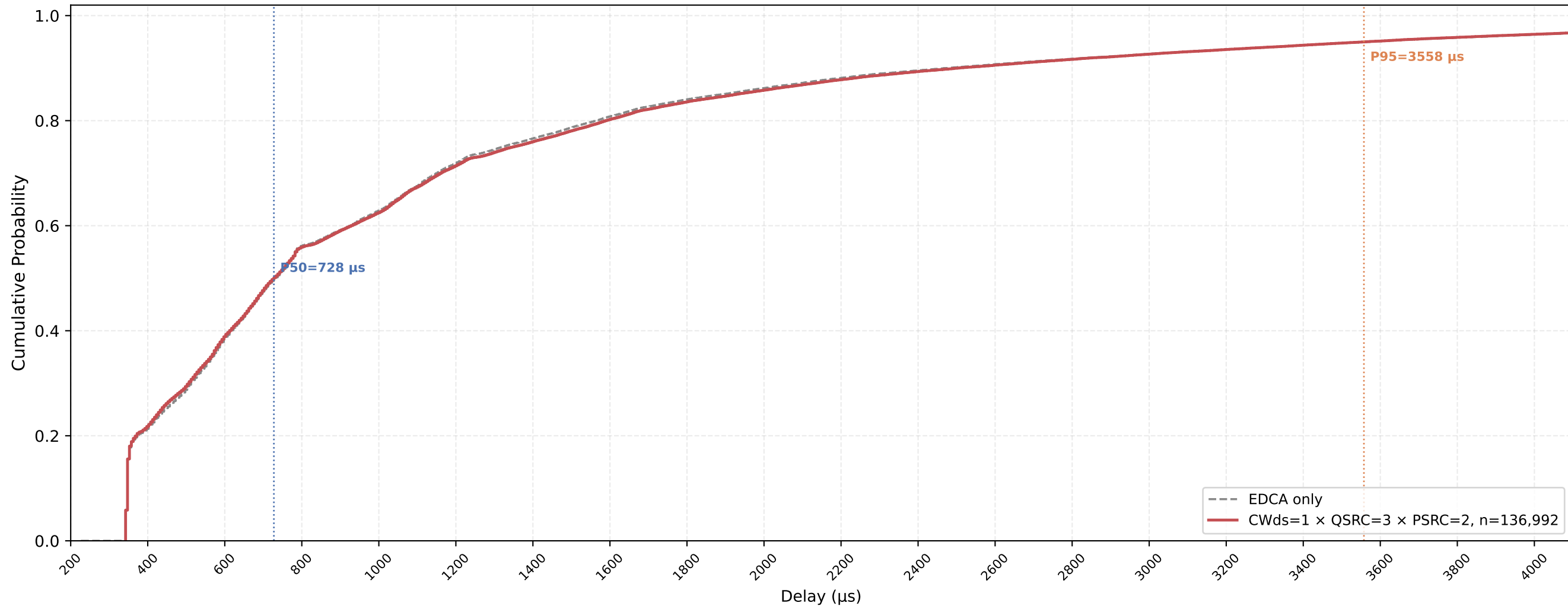
Legacy STA VO Delay CDF — CWds=1 × QSRC=3 × PSRC=2 nSta=30, nPedca=5, 0.5Mbps, avg of 10 runs
