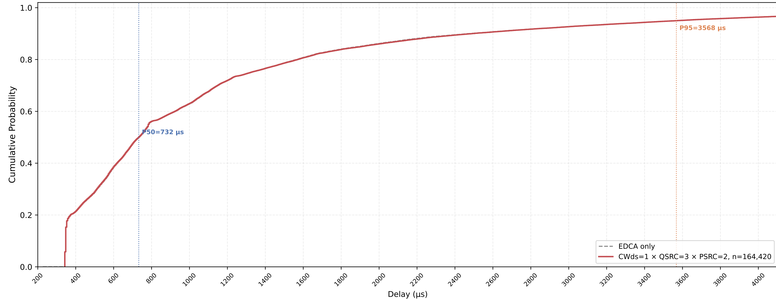
VO (all STAs) Delay CDF — CWds=1 × QSRC=3 × PSRC=2 nSta=30, nPedca=5, 0.5Mbps, avg of 10 runs
