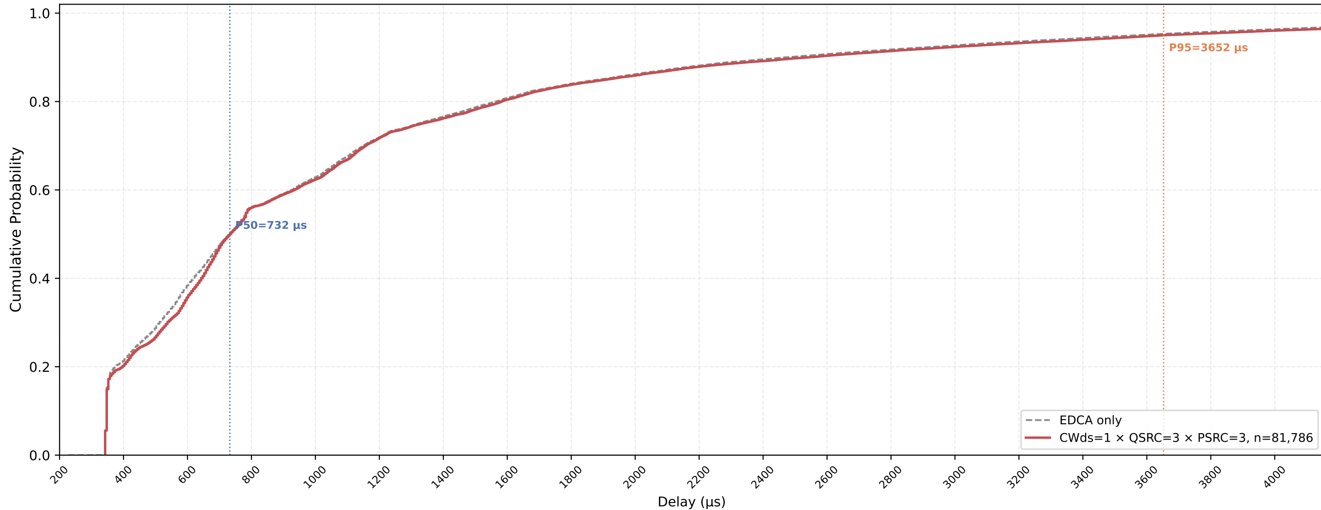
Legacy STA VO Delay CDF — CWds=1 × QSRC=3 × PSRC=3 nSta=30, nPedca=15, 0.5Mbps, avg of 10 runs
