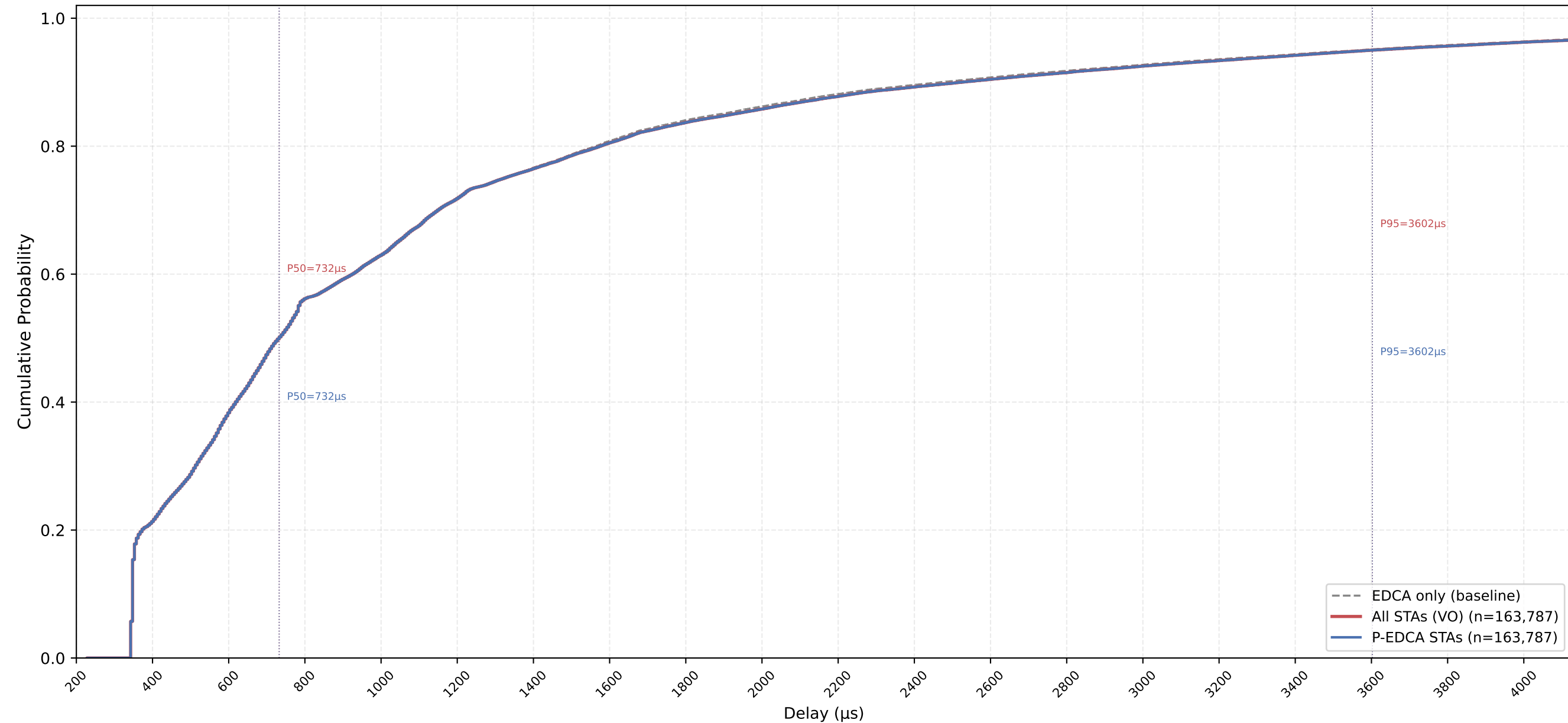
VO Delay CDF — P-EDCA / Legacy / All | CWds=1 × QSRC=4 × PSRC=1 nSta=30, nPedca=30/30, 0.5Mbps, avg of 10 runs
