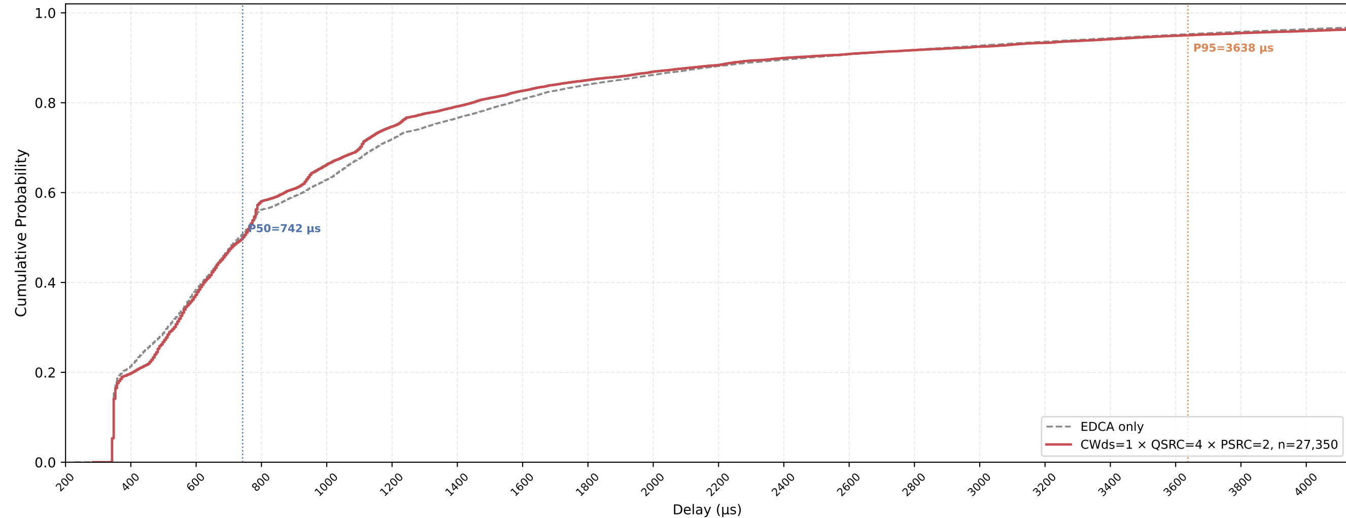
P-EDCA STA VO Delay CDF — CWds=1 × QSRC=4 × PSRC=2 nSta=30, nPedca=5, 0.5Mbps, avg of 10 runs
