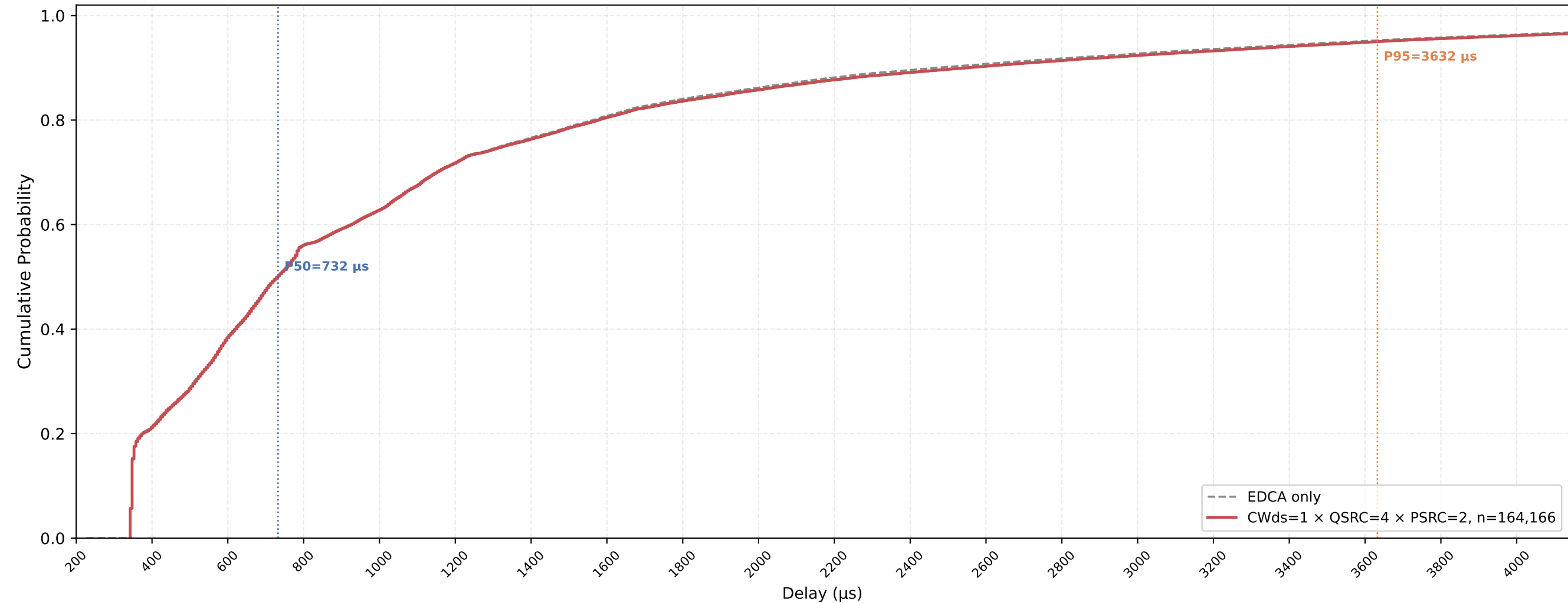
P-EDCA STA VO Delay CDF — CWds=1 × QSRC=4 × PSRC=2 nSta=30, nPedca=30, 0.5Mbps, avg of 10 runs
