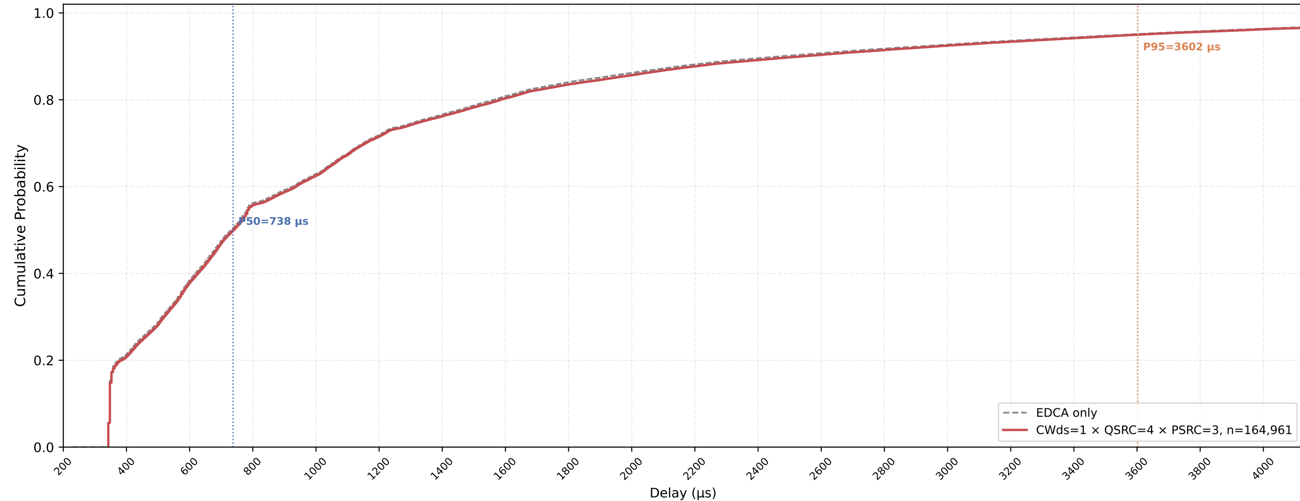
VO (all STAs) Delay CDF — CWds=1 × QSRC=4 × PSRC=3 nSta=30, nPedca=15, 0.5Mbps, avg of 10 runs
