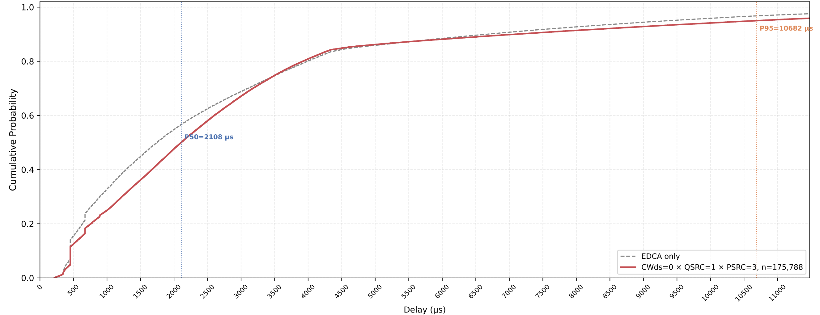
VO (all STAs) Delay CDF — CWds=0 × QSRC=1 × PSRC=3 nSta=30, nPedca=15, 1Mbps, avg of 10 runs
