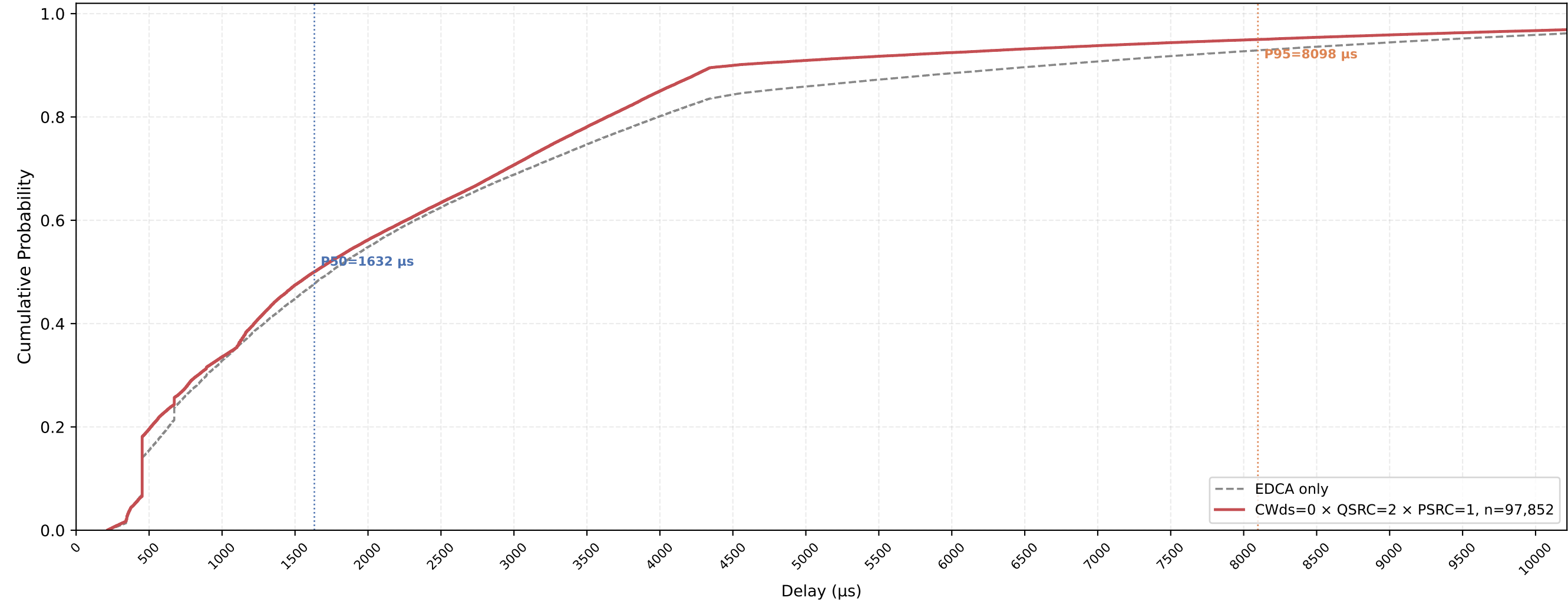
P-EDCA STA VO Delay CDF — CWds=0 × QSRC=2 × PSRC=1 nSta=30, nPedca=15, 1Mbps, avg of 10 runs
