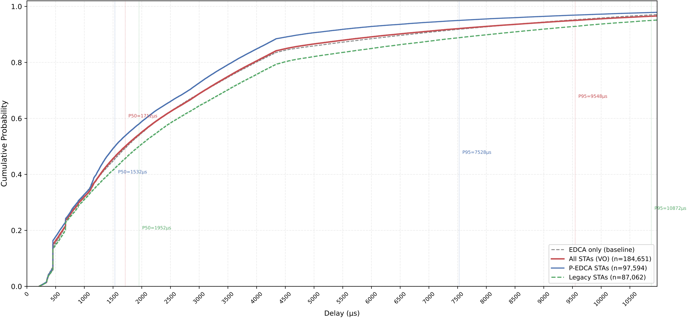
VO Delay CDF — P-EDCA / Legacy / All | CWds=1 × QSRC=3 × PSRC=1 nSta=30, nPedca=15/30, 1Mbps, avg of 10 runs
