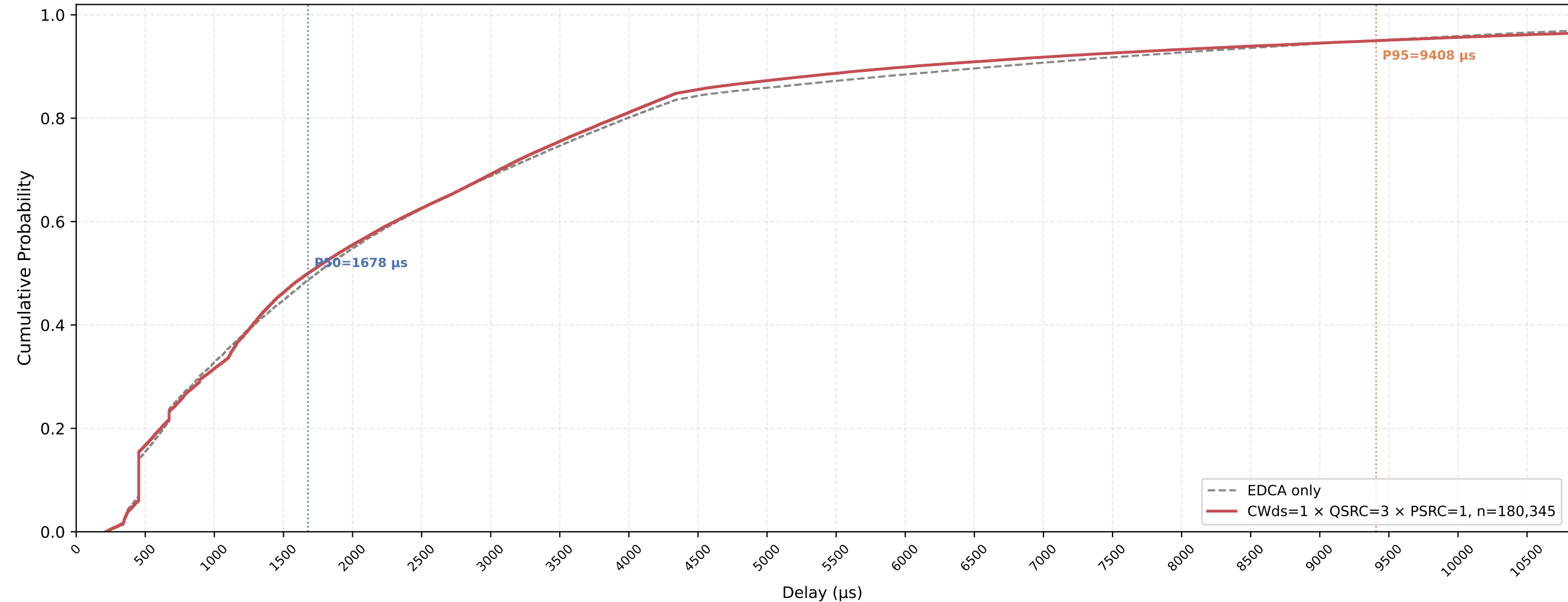
VO (all STAs) Delay CDF — CWds=1 × QSRC=3 × PSRC=1 nSta=30, nPedca=30, 1Mbps, avg of 10 runs
