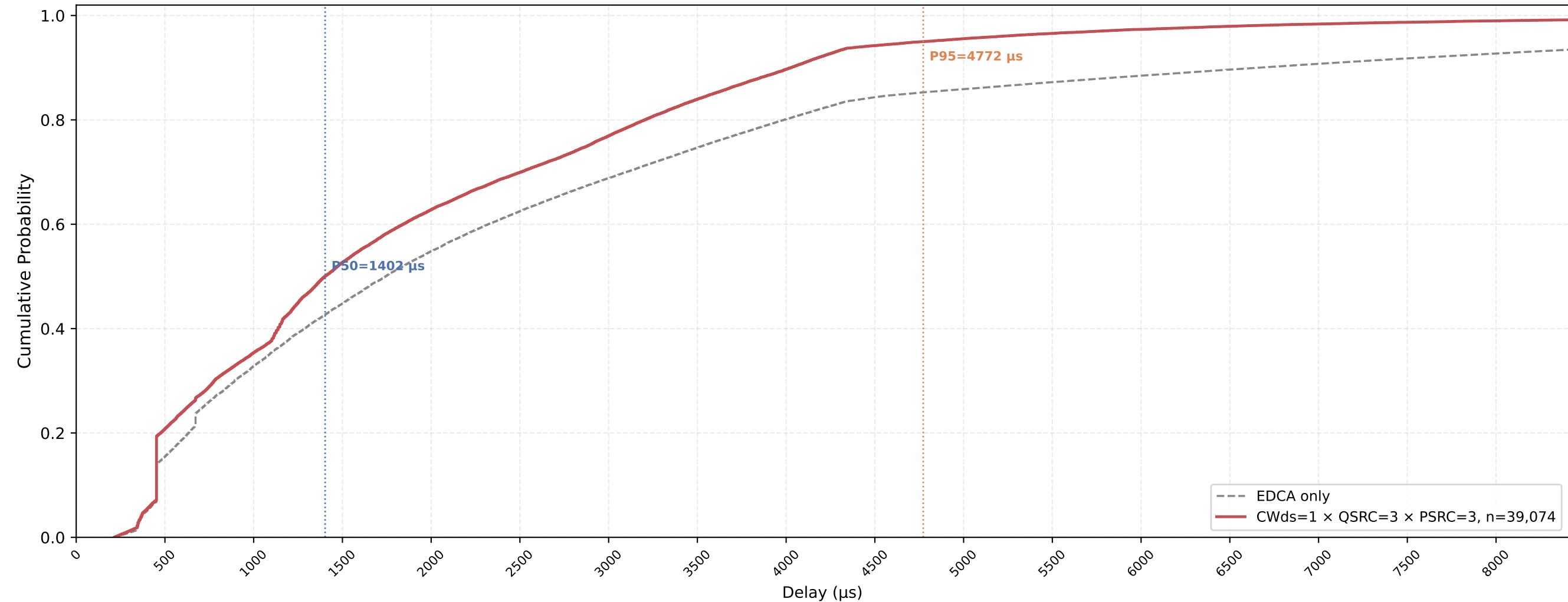
P-EDCA STA VO Delay CDF — CWds=1 × QSRC=3 × PSRC=3 nSta=30, nPedca=5, 1Mbps, avg of 10 runs
