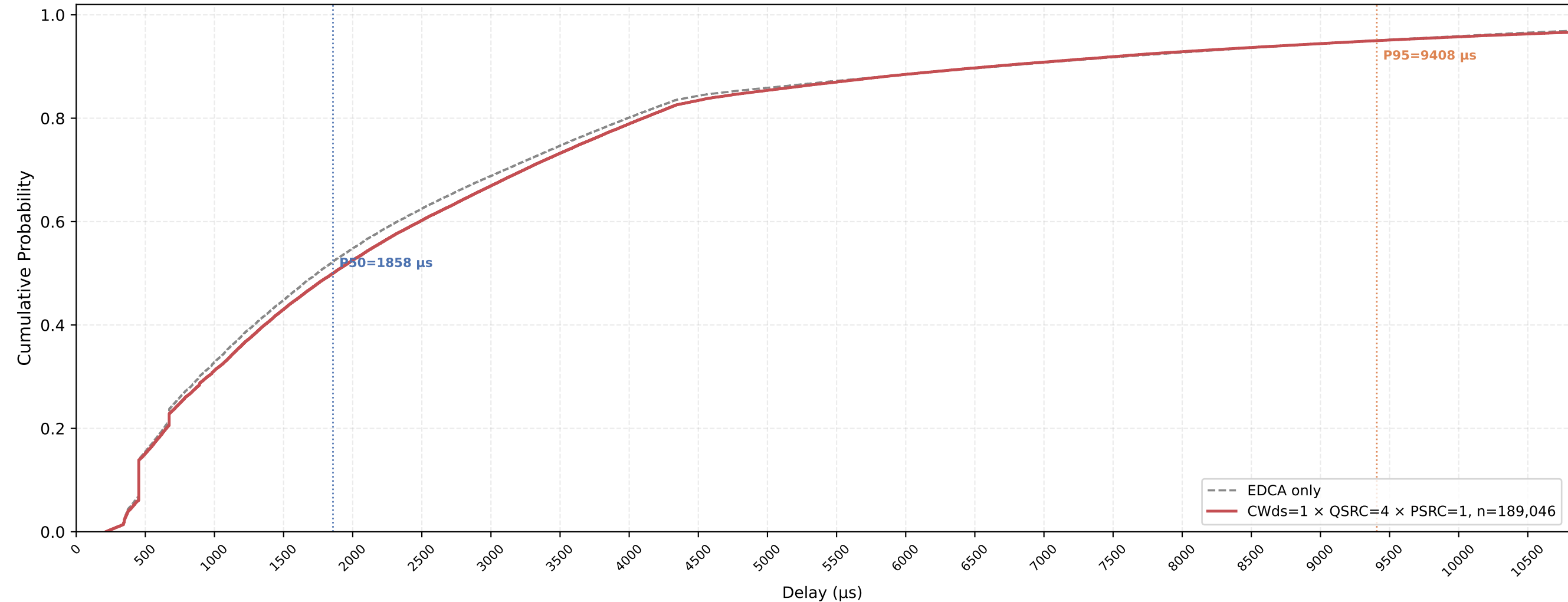
VO (all STAs) Delay CDF — CWds=1 × QSRC=4 × PSRC=1 nSta=30, nPedca=15, 1Mbps, avg of 10 runs
