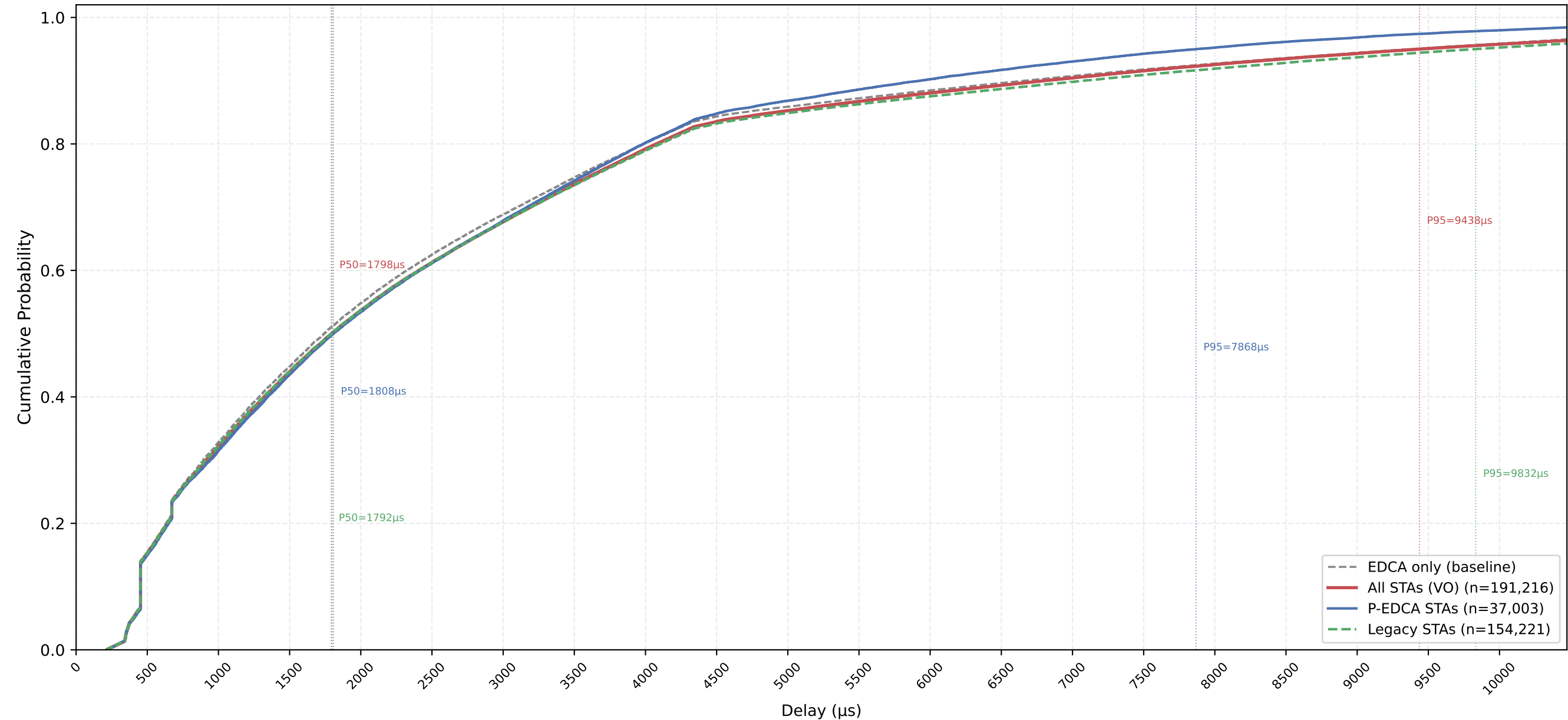
VO Delay CDF — P-EDCA / Legacy / All | CWds=1 × QSRC=5 × PSRC=2 nSta=30, nPedca=5/30, 1Mbps, avg of 10 runs
