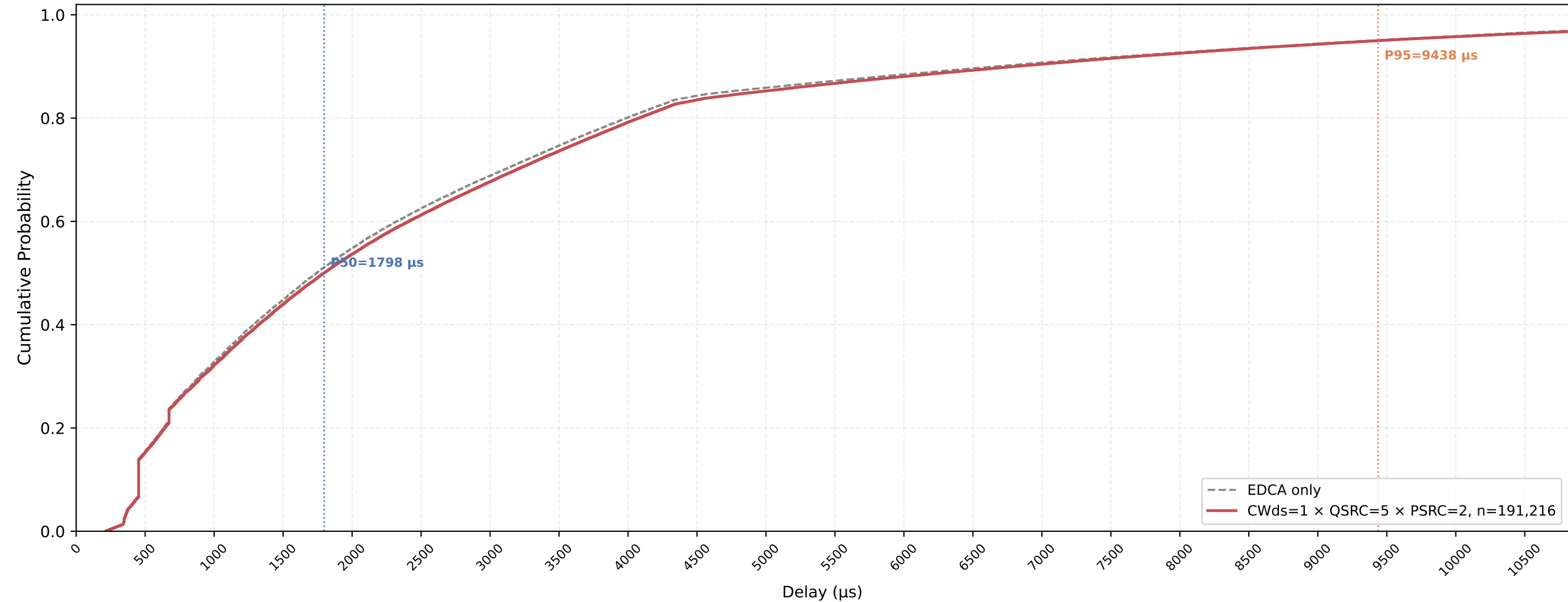
VO (all STAs) Delay CDF — CWds=1 × QSRC=5 × PSRC=2 nSta=30, nPedca=5, 1Mbps, avg of 10 runs
