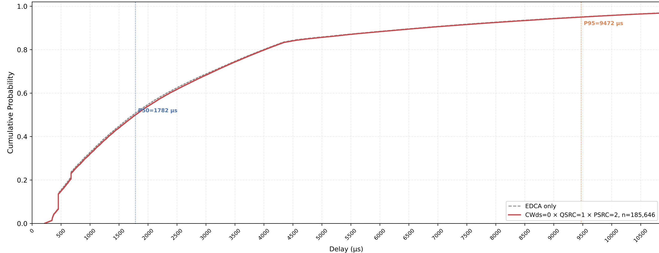
VO (all STAs) Delay CDF — CWds=0 × QSRC=1 × PSRC=2 nSta=30, nPedca=15, 1Mbps, avg of 10 runs
