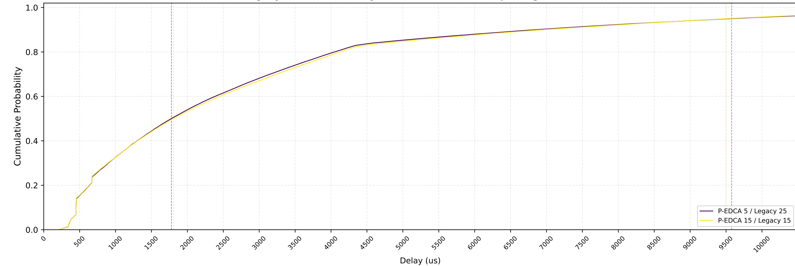
Legacy EDCA STAs Delay CDF — nSta=30, 1Mbps, avg of 10 runs
