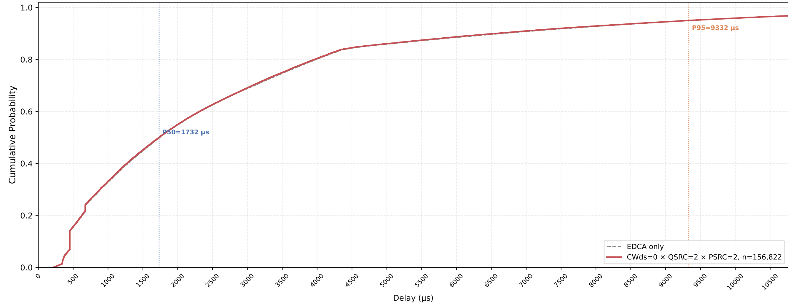
Legacy STA VO Delay CDF — CWds=0 × QSRC=2 × PSRC=2 nSta=30, nPedca=5, 1Mbps, avg of 10 runs
