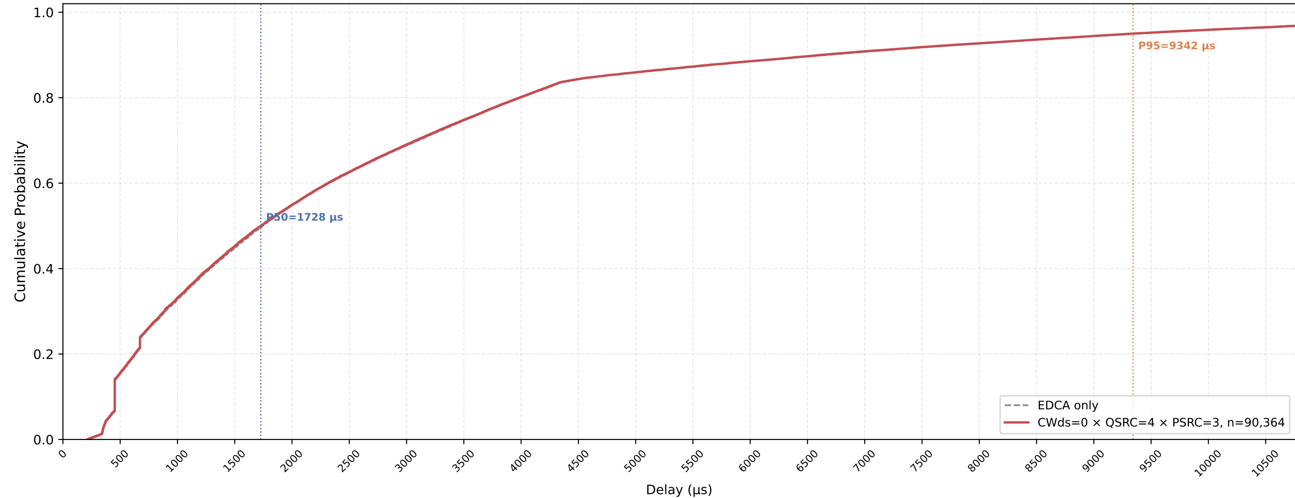
Legacy STA VO Delay CDF — CWds=0 × QSRC=4 × PSRC=3 nSta=30, nPedca=15, 1Mbps, avg of 10 runs
