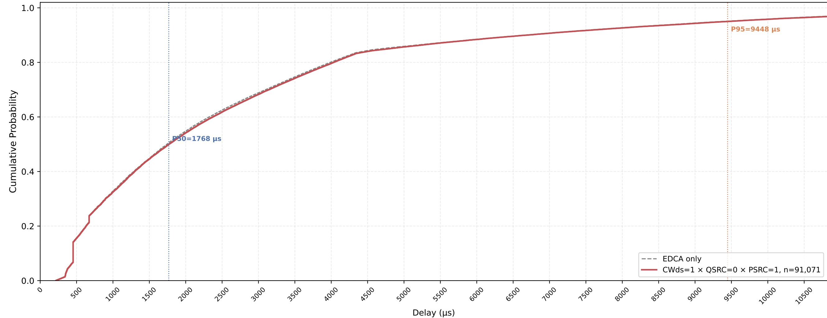
Legacy STA VO Delay CDF — CWds=1 × QSRC=0 × PSRC=1 nSta=30, nPedca=15, 1Mbps, avg of 10 runs
