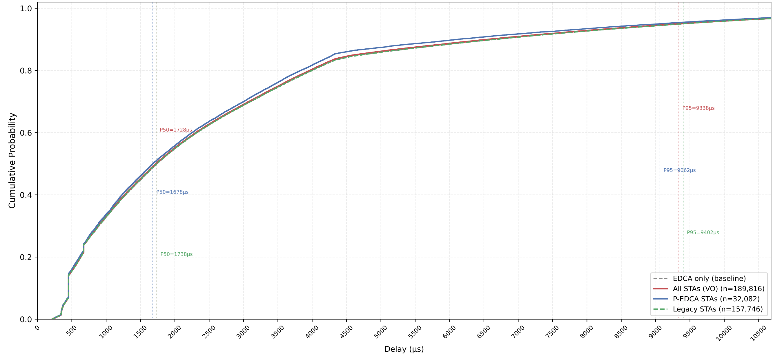
VO Delay CDF — P-EDCA / Legacy / All | CWds=1 × QSRC=2 × PSRC=1 nSta=30, nPedca=5/30, 1Mbps, avg of 10 runs
