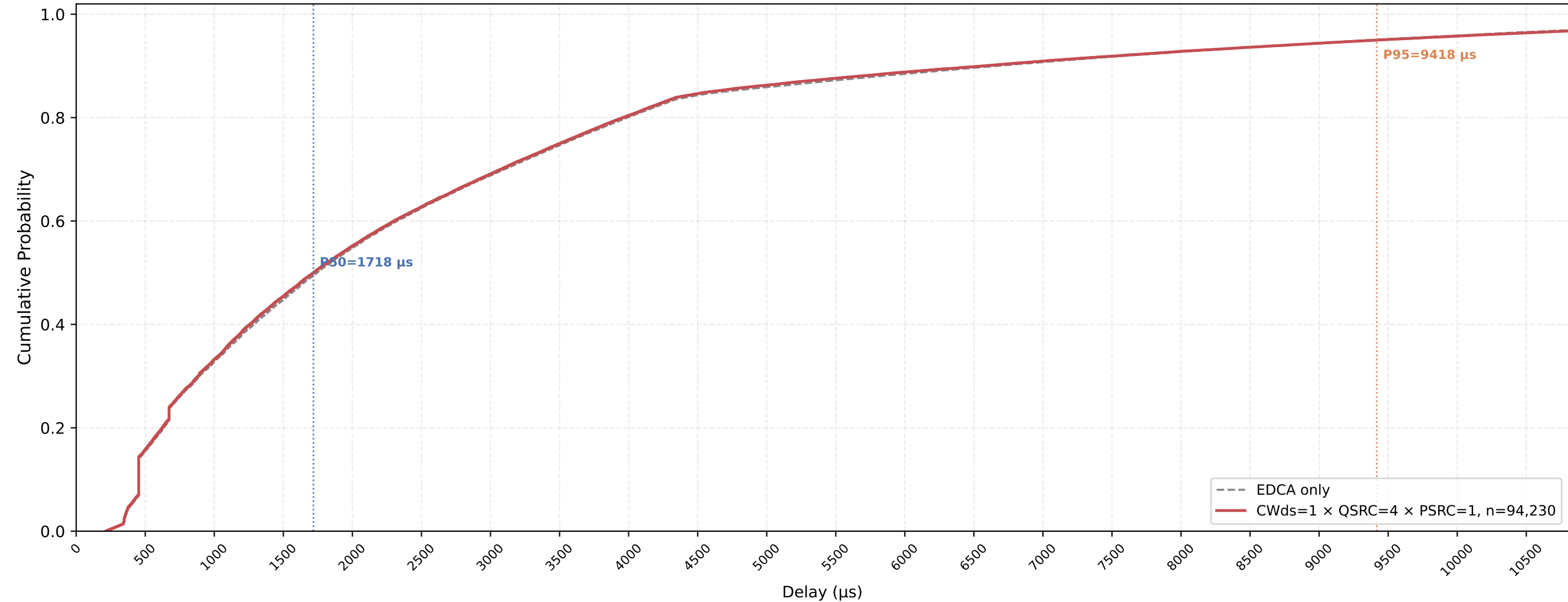
P-EDCA STA VO Delay CDF — CWds=1 × QSRC=4 × PSRC=1 nSta=30, nPedca=15, 1Mbps, avg of 10 runs
