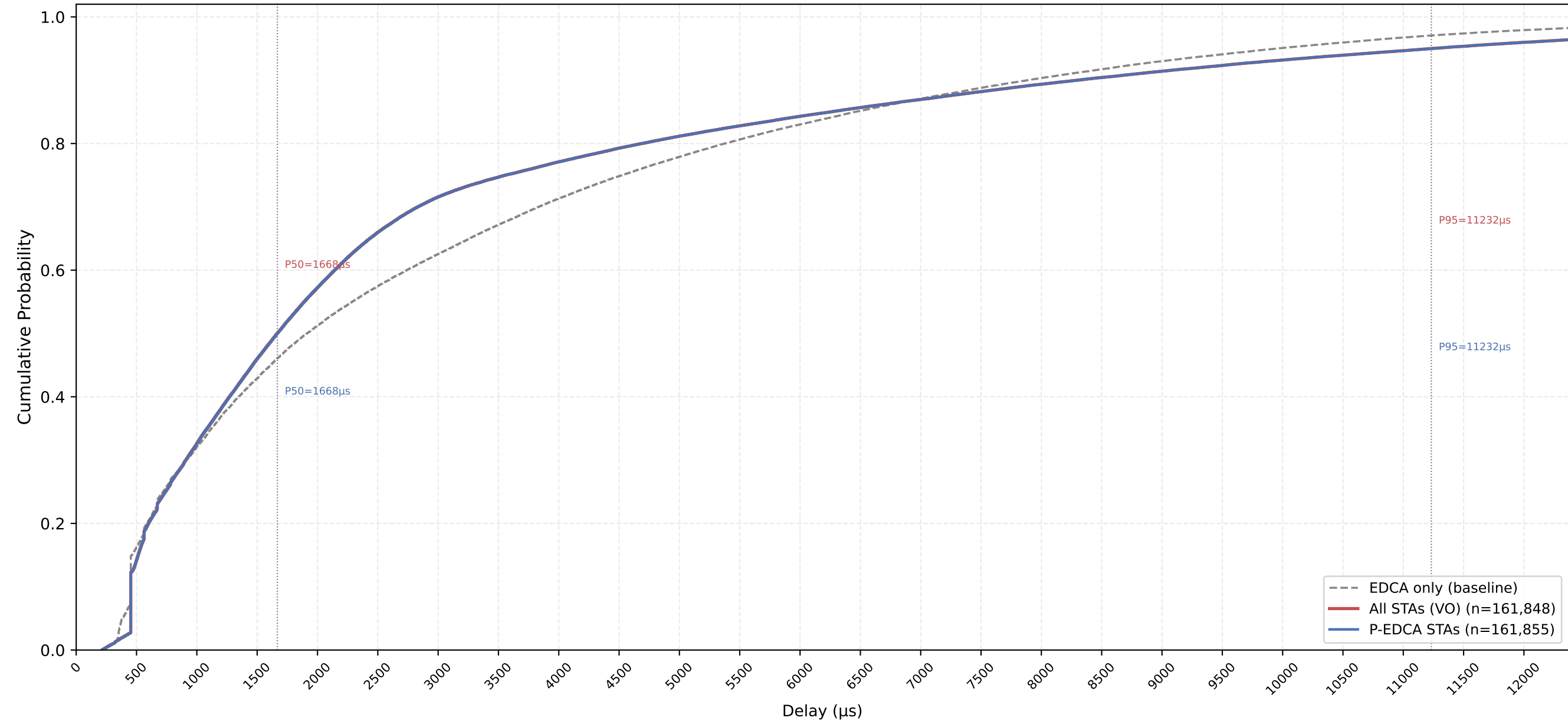
VO Delay CDF — P-EDCA / Legacy / All | CWds=0 × QSRC=0 × PSRC=1 nSta=30, nPedca=30/30, 1Mbps, avg of 10 runs
