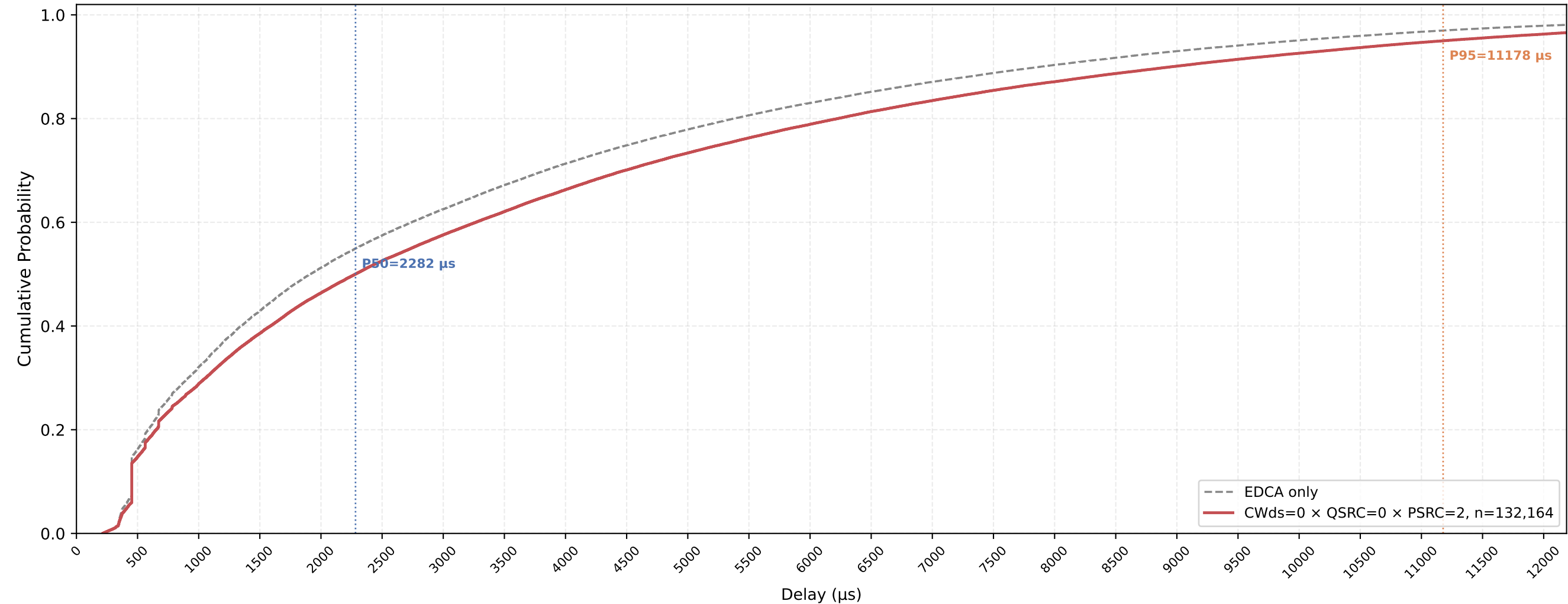
Legacy STA VO Delay CDF — CWds=0 × QSRC=0 × PSRC=2 nSta=30, nPedca=5, 1Mbps, avg of 10 runs
