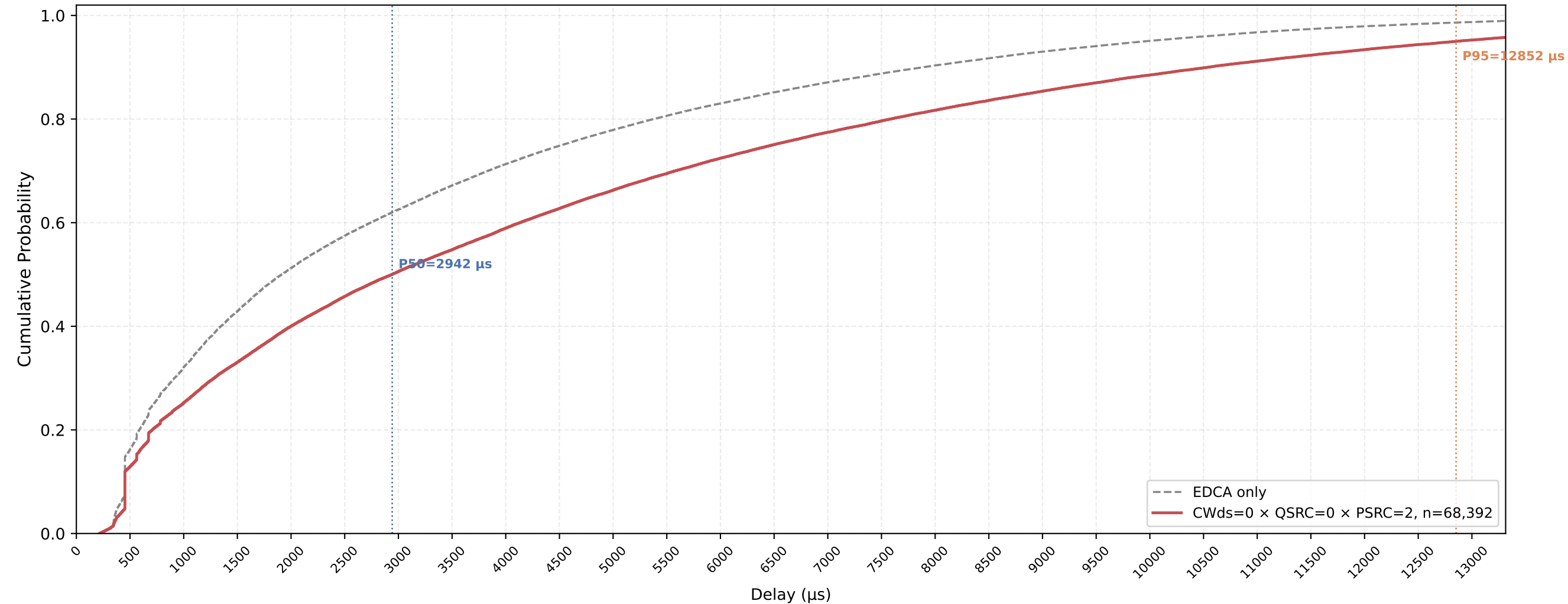
Legacy STA VO Delay CDF — CWds=0 × QSRC=0 × PSRC=2 nSta=30, nPedca=15, 1Mbps, avg of 10 runs
