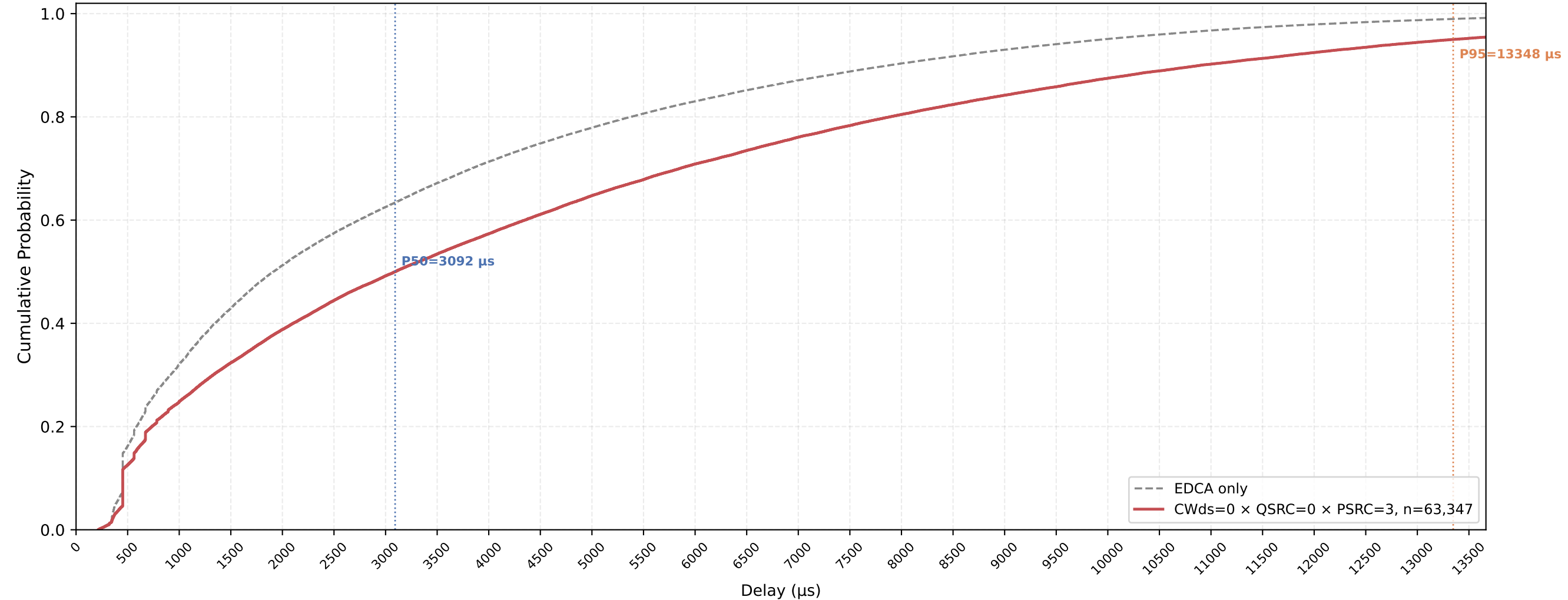
Legacy STA VO Delay CDF — CWds=0 × QSRC=0 × PSRC=3 nSta=30, nPedca=15, 1Mbps, avg of 10 runs
