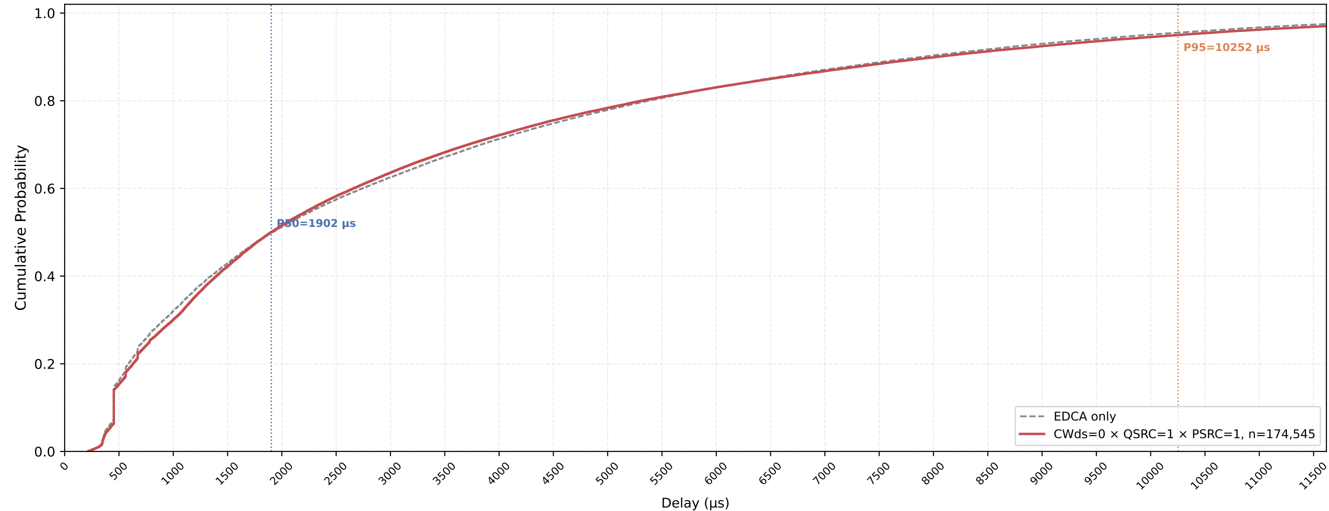
VO (all STAs) Delay CDF — CWds=0 × QSRC=1 × PSRC=1 nSta=30, nPedca=5, 1Mbps, avg of 10 runs
