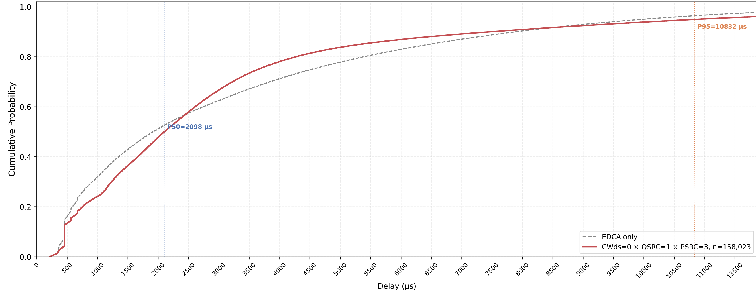
P-EDCA STA VO Delay CDF — CWds=0 × QSRC=1 × PSRC=3 nSta=30, nPedca=30, 1Mbps, avg of 10 runs
