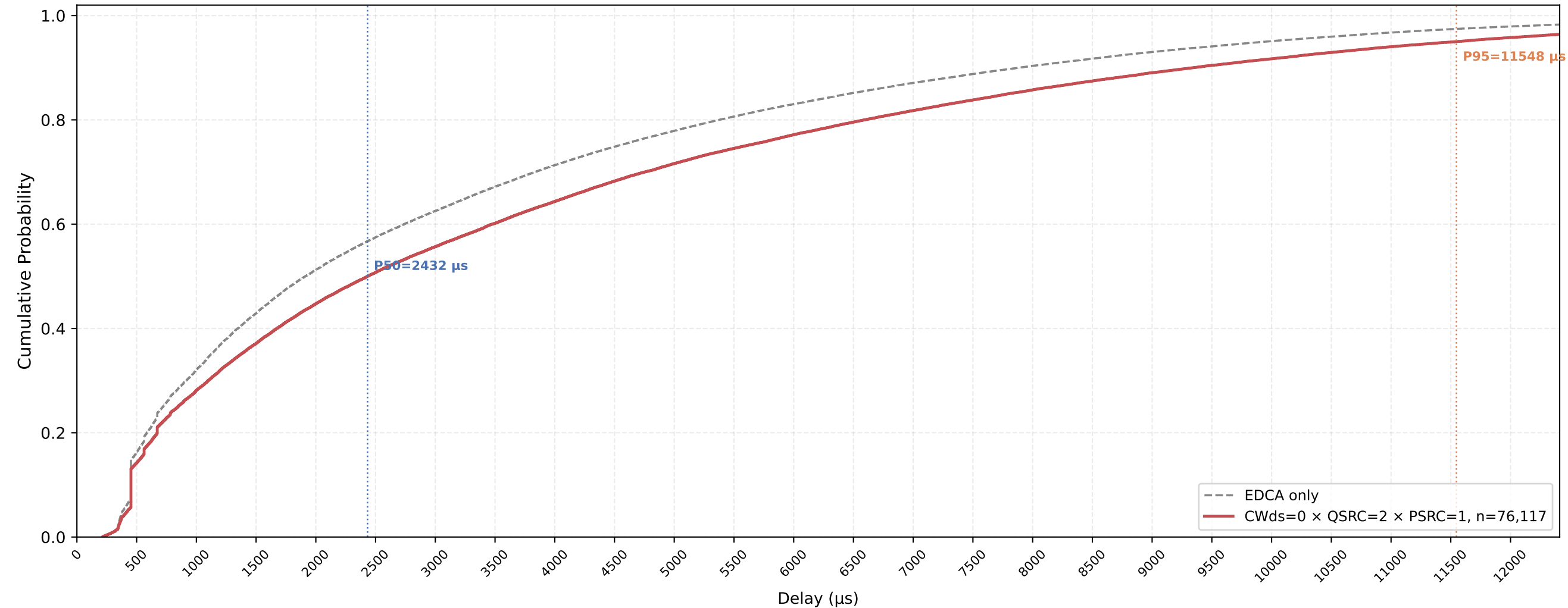
Legacy STA VO Delay CDF — CWds=0 × QSRC=2 × PSRC=1 nSta=30, nPedca=15, 1Mbps, avg of 10 runs
