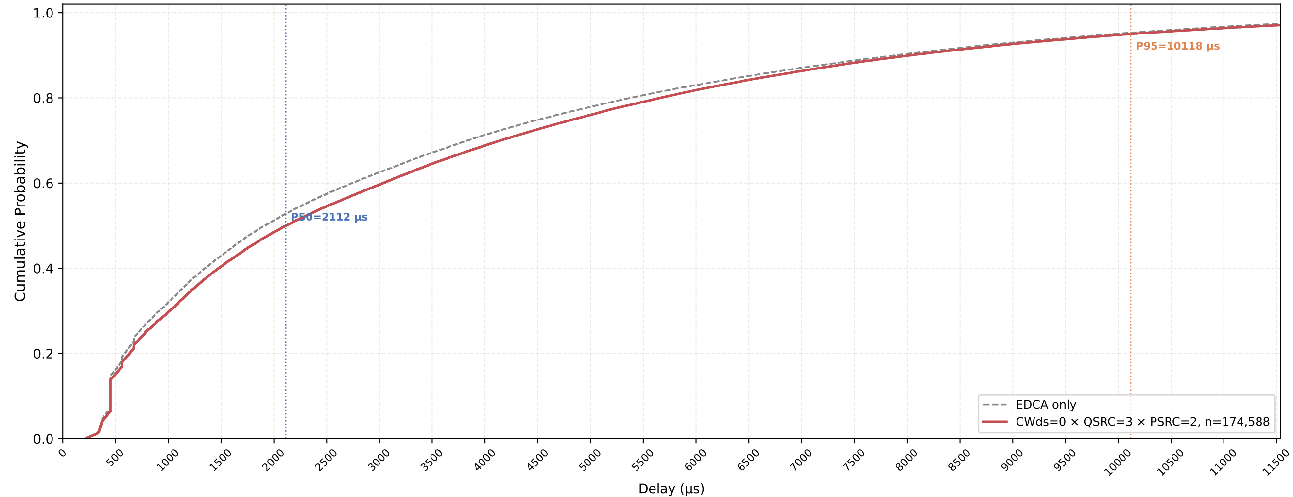
VO (all STAs) Delay CDF — CWds=0 × QSRC=3 × PSRC=2 nSta=30, nPedca=5, 1Mbps, avg of 10 runs
