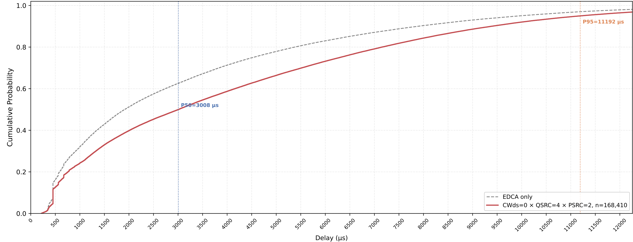
P-EDCA STA VO Delay CDF — CWds=0 × QSRC=4 × PSRC=2 nSta=30, nPedca=30, 1Mbps, avg of 10 runs
