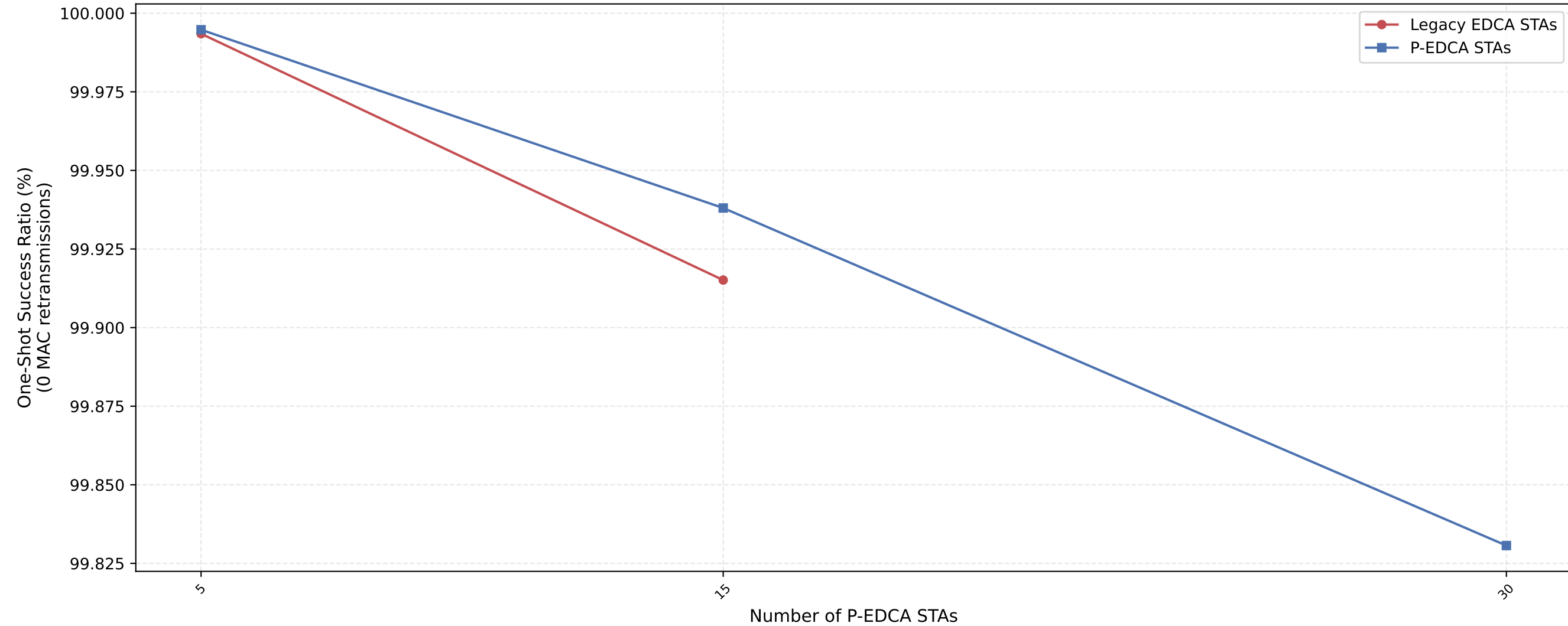
EDCA One-Shot Success Ratio (0 retx) — nSta=30, 1Mbps (avg of 10 runs)
