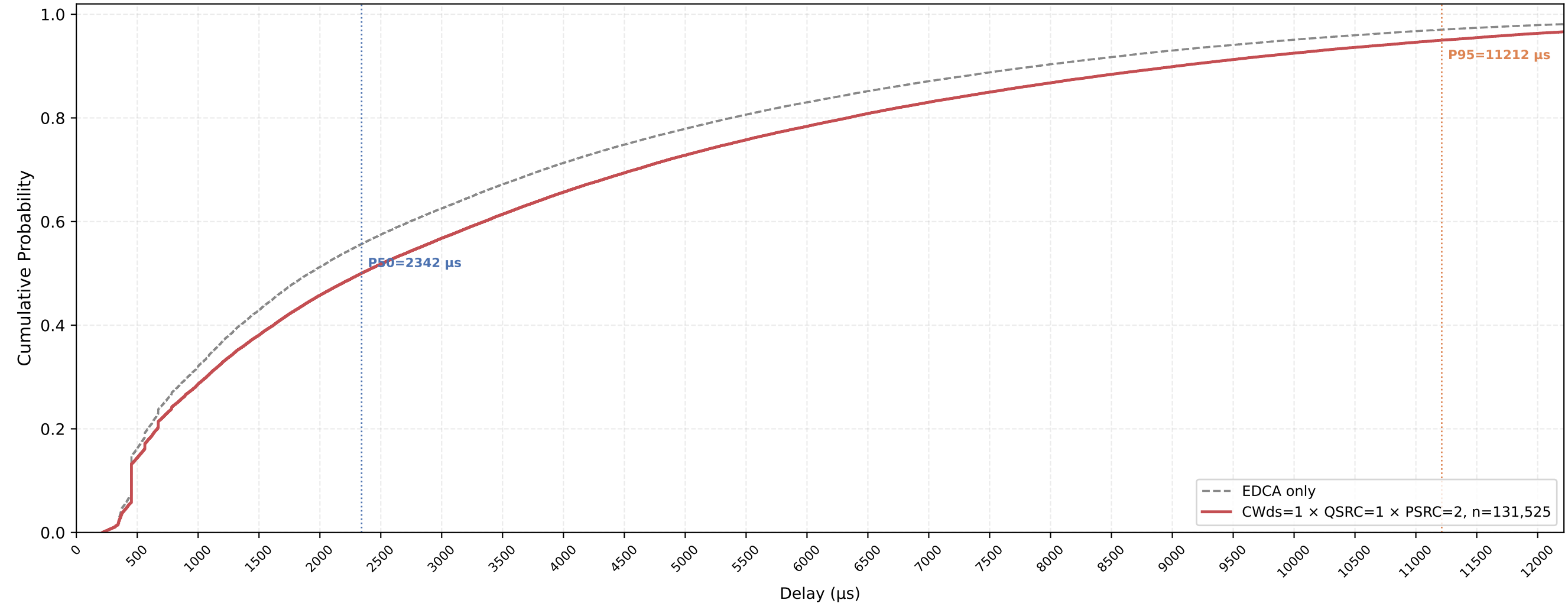
Legacy STA VO Delay CDF — CWds=1 × QSRC=1 × PSRC=2 nSta=30, nPedca=5, 1Mbps, avg of 10 runs
