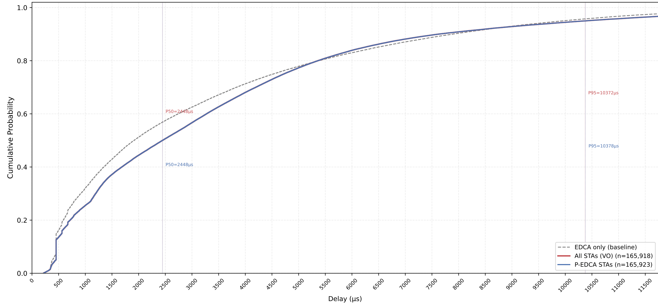
VO Delay CDF — P-EDCA / Legacy / All | CWds=1 × QSRC=2 × PSRC=1 nSta=30, nPedca=30/30, 1Mbps, avg of 10 runs
