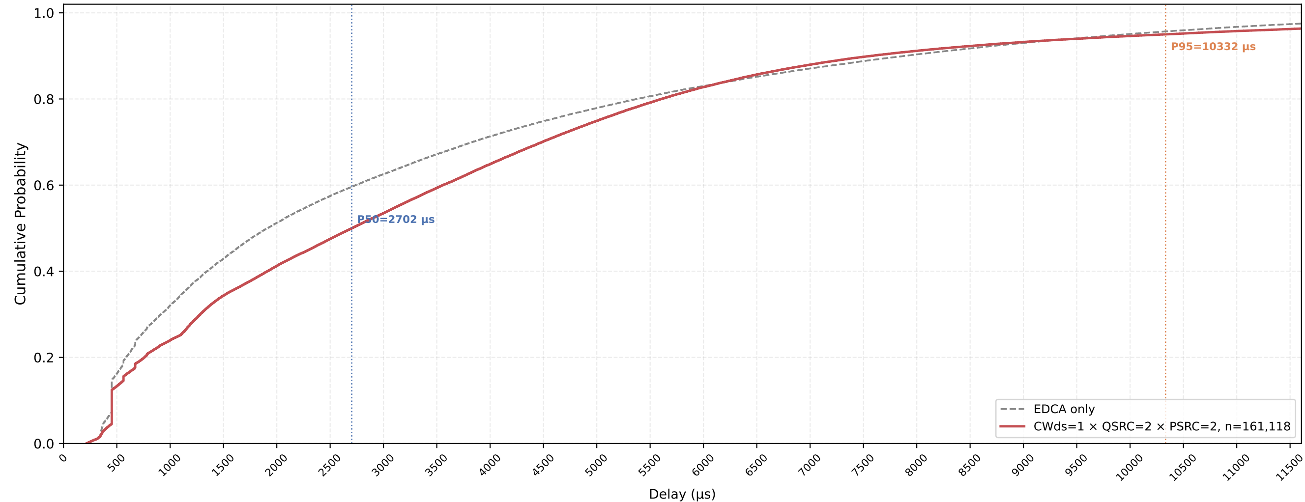
VO (all STAs) Delay CDF — CWds=1 × QSRC=2 × PSRC=2 nSta=30, nPedca=30, 1Mbps, avg of 10 runs
