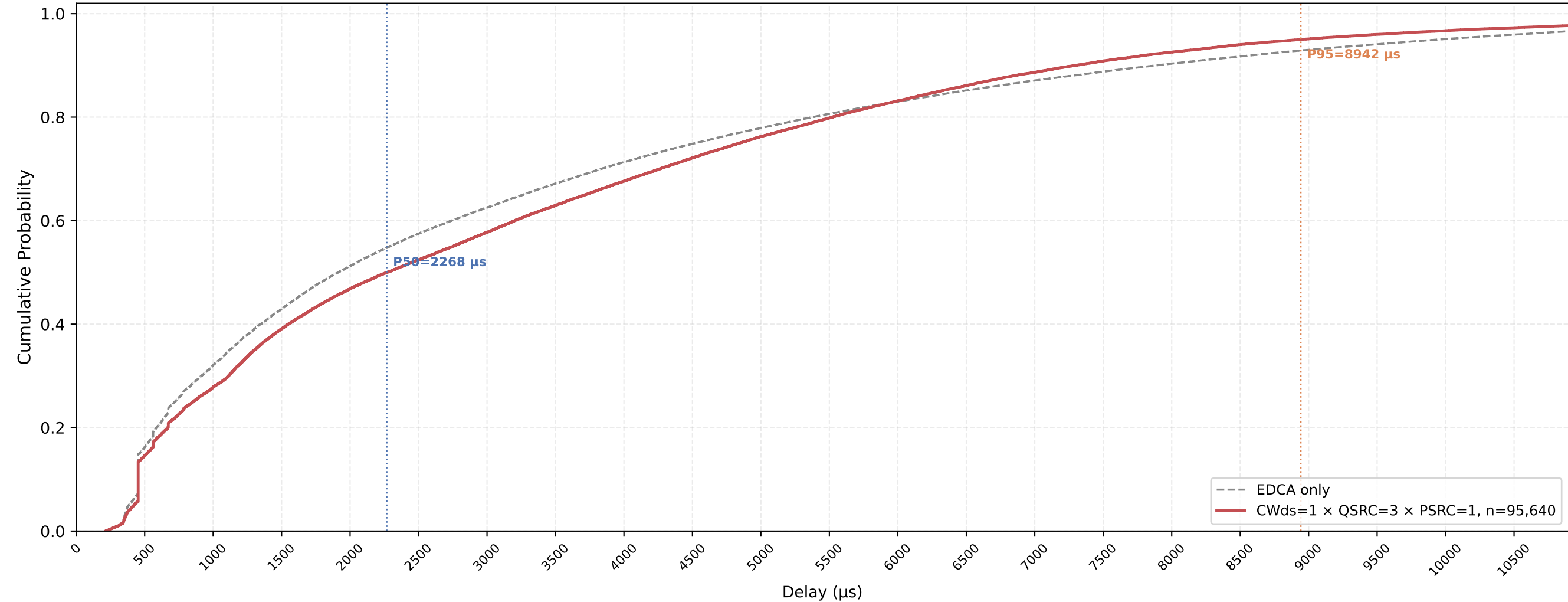
P-EDCA STA VO Delay CDF — CWds=1 × QSRC=3 × PSRC=1 nSta=30, nPedca=15, 1Mbps, avg of 10 runs
