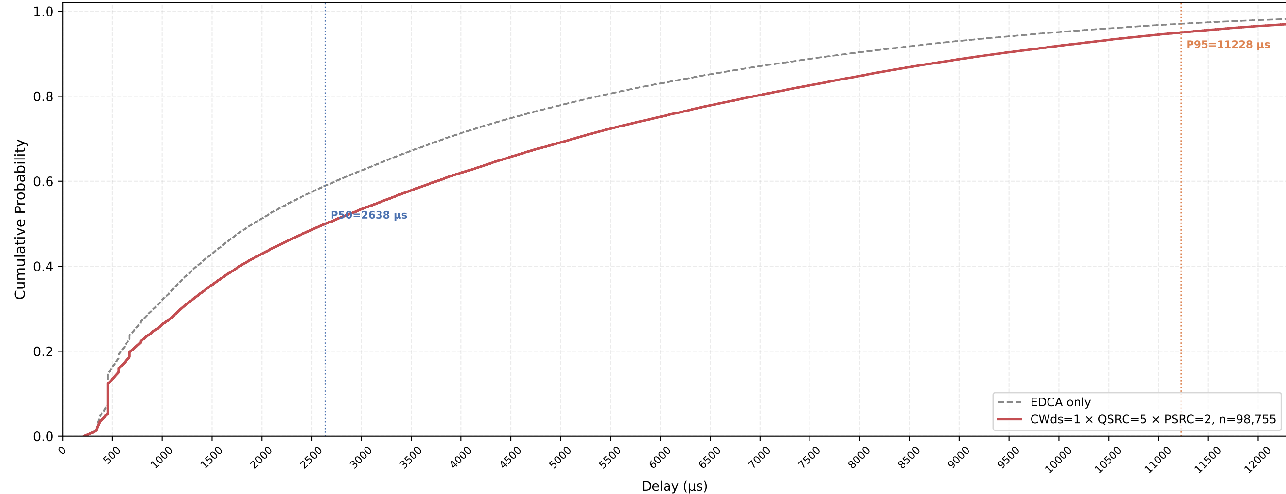
P-EDCA STA VO Delay CDF — CWds=1 × QSRC=5 × PSRC=2 nSta=30, nPedca=15, 1Mbps, avg of 10 runs
