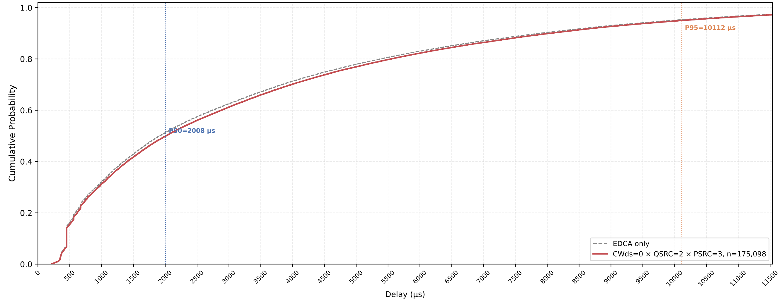
VO (all STAs) Delay CDF — CWds=0 × QSRC=2 × PSRC=3 nSta=30, nPedca=5, 1Mbps, avg of 10 runs
