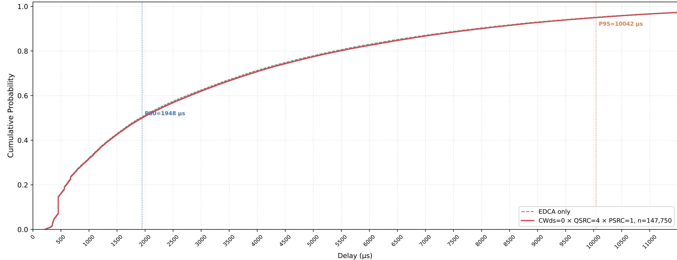
Legacy STA VO Delay CDF — CWds=0 × QSRC=4 × PSRC=1 nSta=30, nPedca=5, 1Mbps, avg of 10 runs
