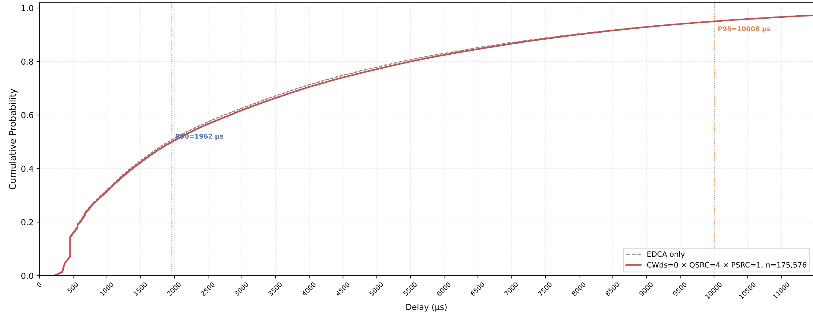
VO (all STAs) Delay CDF — CWds=0 × QSRC=4 × PSRC=1 nSta=30, nPedca=15, 1Mbps, avg of 10 runs
