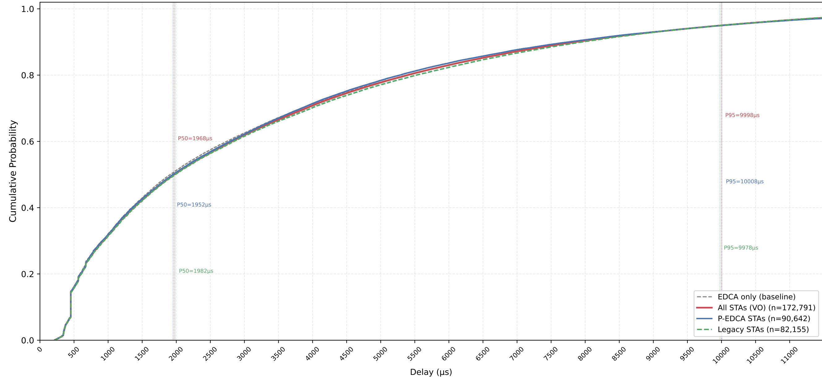
VO Delay CDF — P-EDCA / Legacy / All | CWds=1 × QSRC=2 × PSRC=2 nSta=30, nPedca=15/30, 1Mbps, avg of 10 runs
