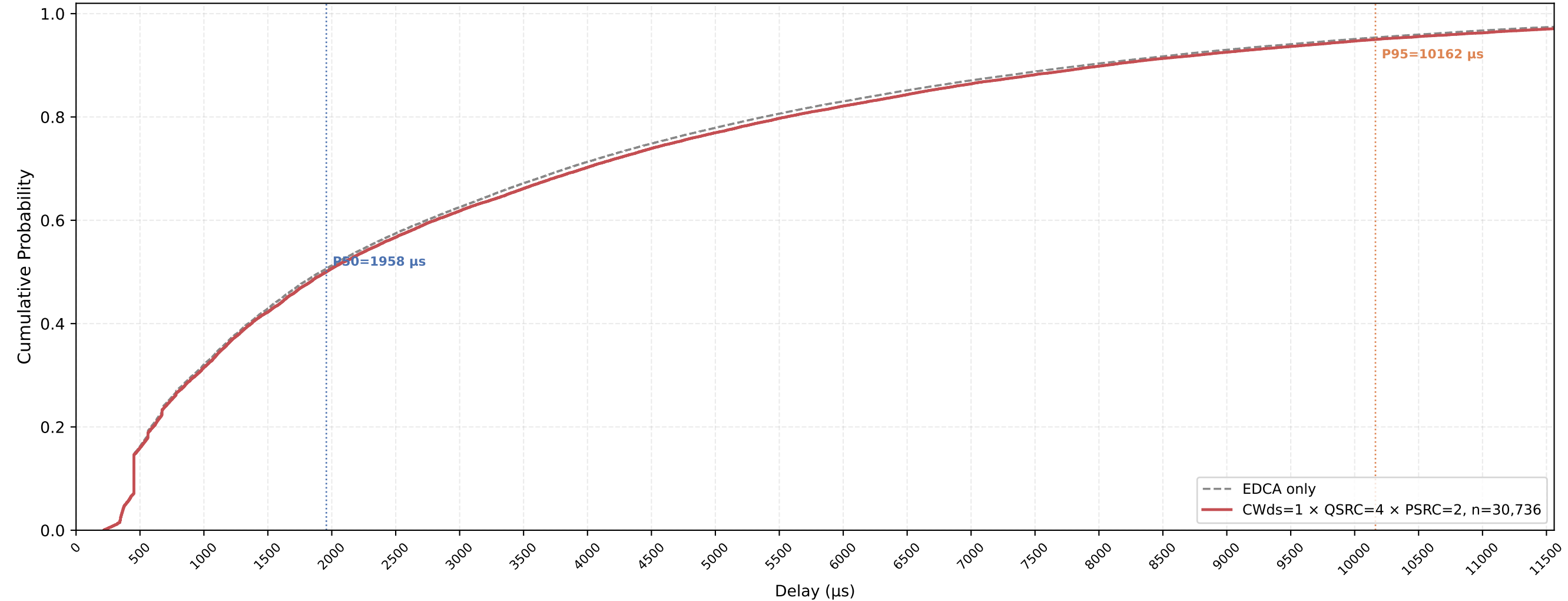
P-EDCA STA VO Delay CDF — CWds=1 × QSRC=4 × PSRC=2 nSta=30, nPedca=5, 1Mbps, avg of 10 runs
