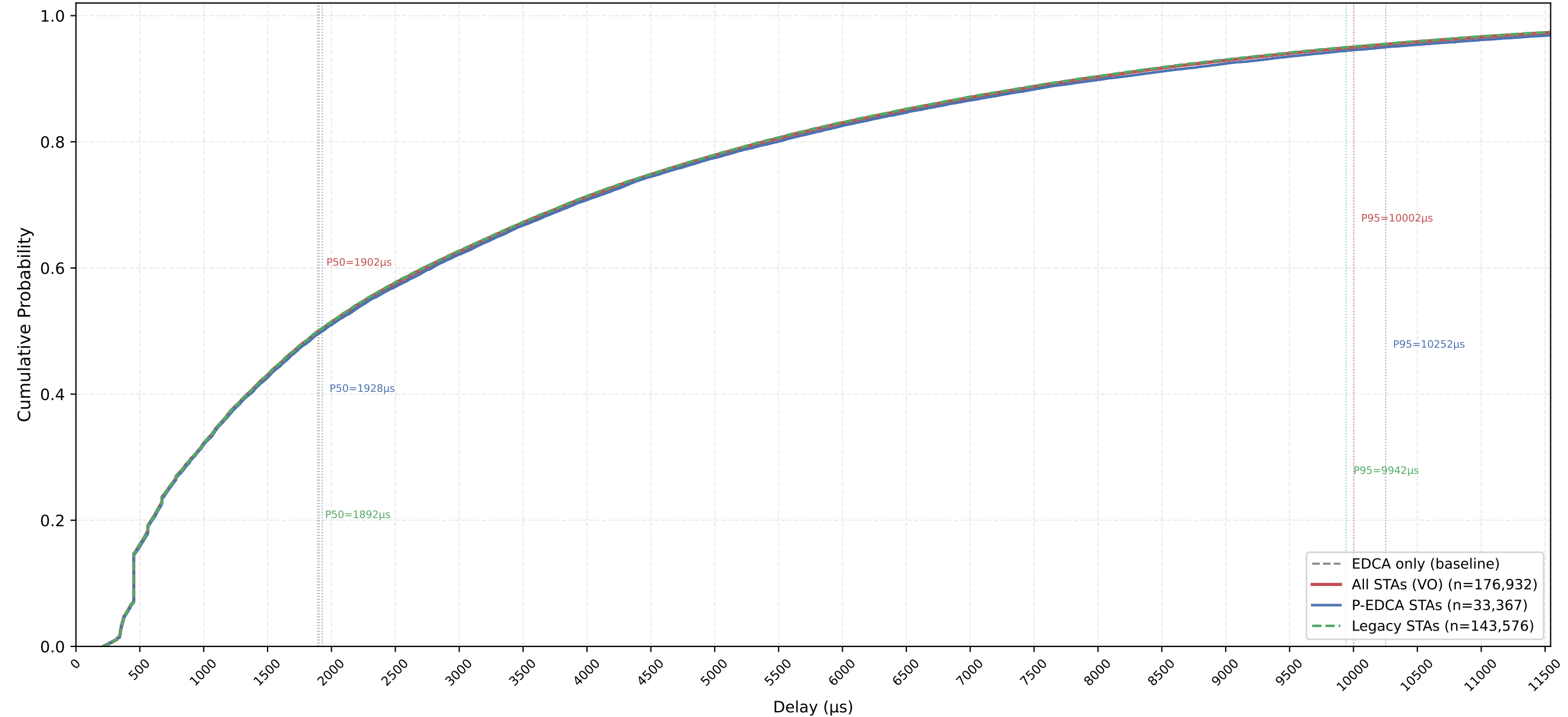
VO Delay CDF — P-EDCA / Legacy / All | CWds=1 × QSRC=4 × PSRC=3 nSta=30, nPedca=5/30, 1Mbps, avg of 10 runs
